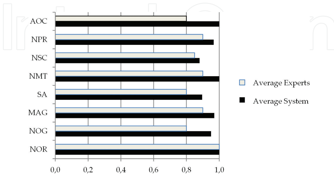
Figure 11. Average values of proactivity measures per agent.
