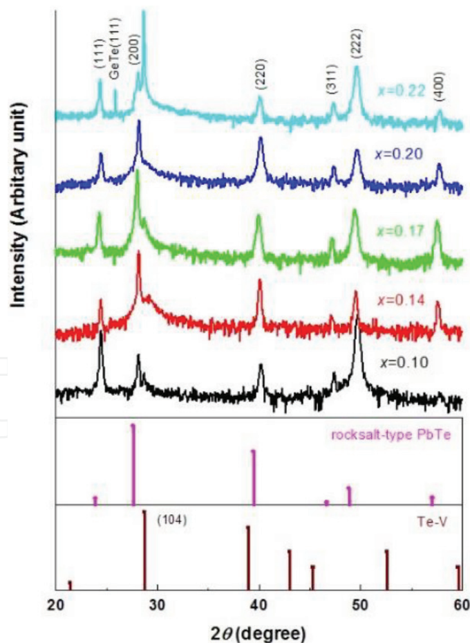
Figure 9. The patterns of XRD analysis for layers evaporated using electron beam heating from ingots with Ge concentration x = 0.10, 0.14, 0.17, 0.20, and 0.22 (ref. [43], reuse permission obtained from Elsevier).
