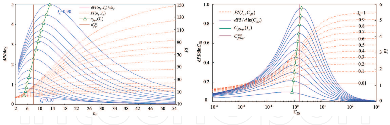
Figure 11. Prediction of productivity performance at different proppant number.
