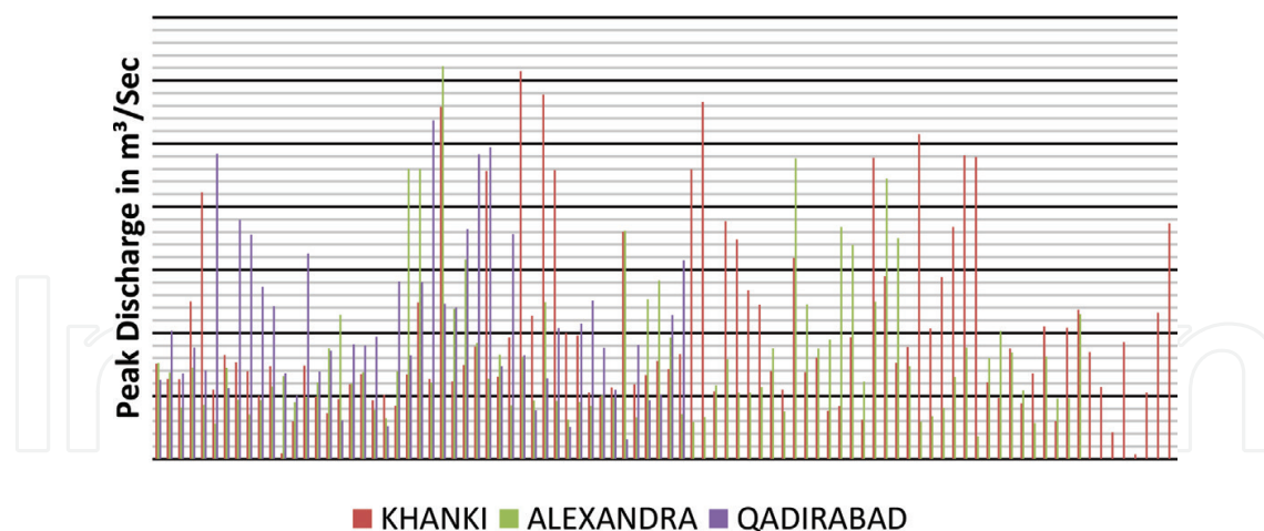
Figure 3. Peak discharge at Khanki Headwork's, Alexandra Headwork's, and Qadirabad Headwork's (1925–2014). Source: [21].
