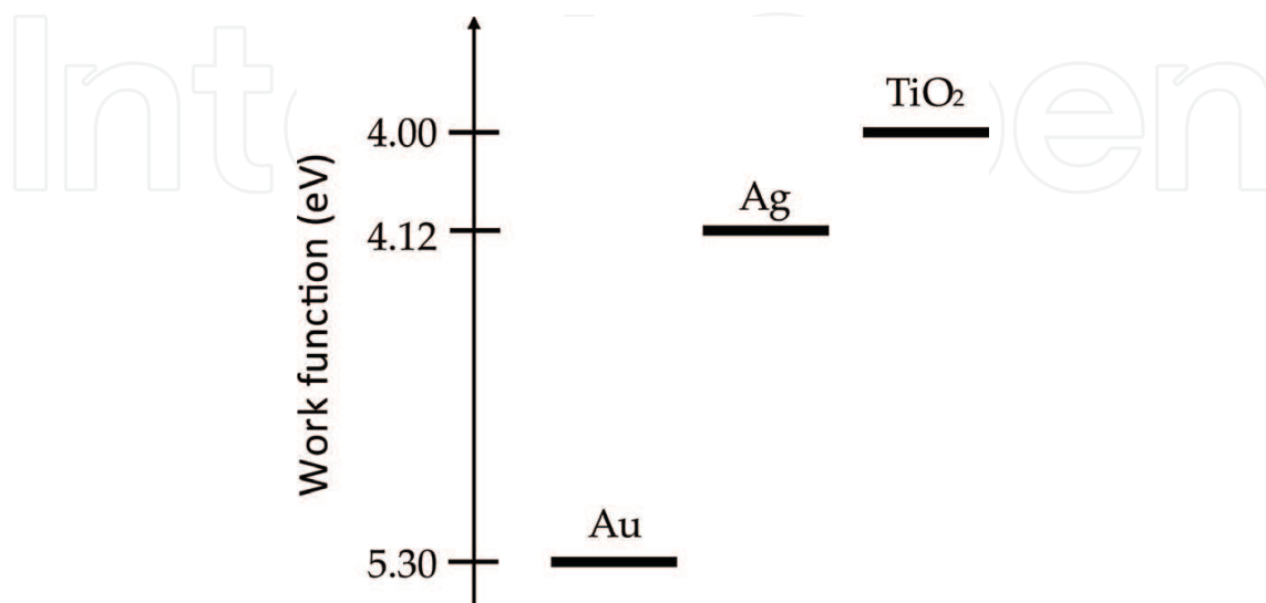
Figure 5. Work function of Au, Ag and TiO 2 .
