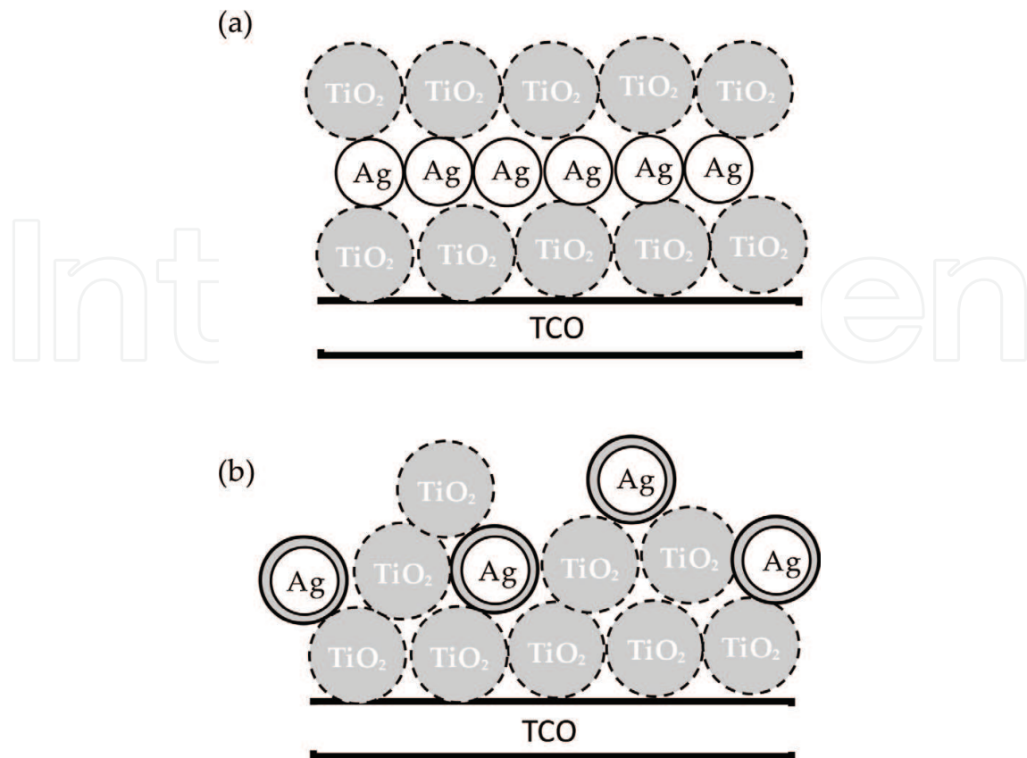
Figure 3. Active layer arrangement to protect metal NPs: (a) \text{TiO}_2/\text{Ag} sandwich structure and (b) metal core-shell.
