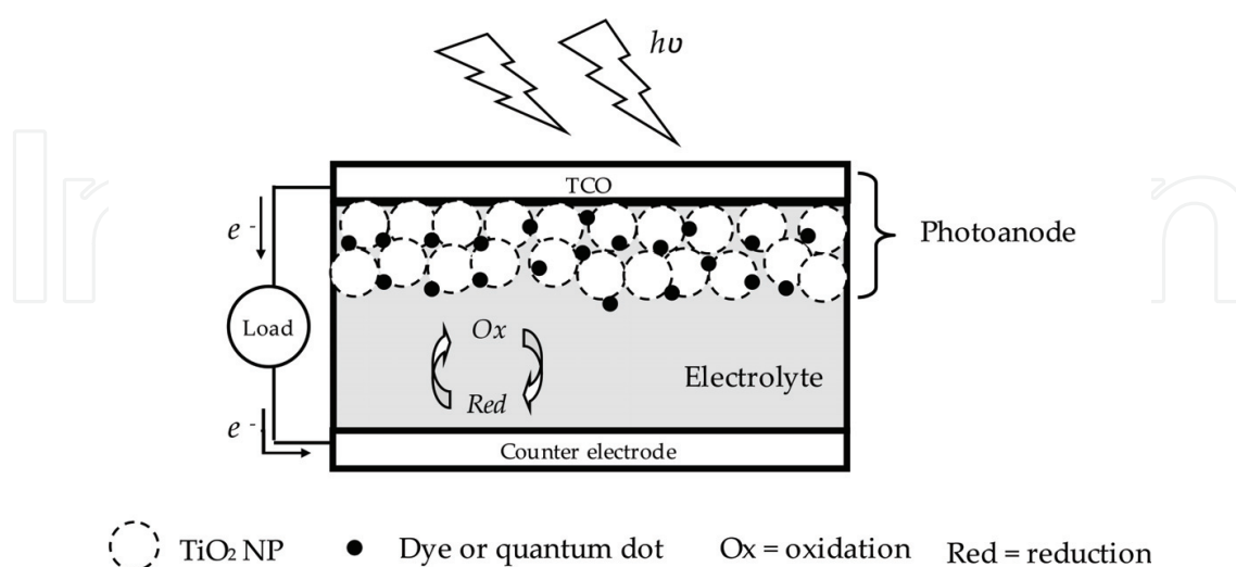
Figure 1. Schematic diagram of DSSC or QDSSC.
