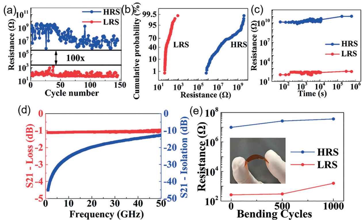
Figure 22. Characteristics of the atomistor. (a, b) Resistance spread of MoS 2 crossbar MIM devices for 150 manual dc switching cycles. (c) Time-dependent measurements of the MoS 2 switch with stable storage of information for a week at room temperature. Resistance of HRS and LRS is determined by measuring the current at a small bias voltage of 0.1 V. The area of this transverse device 2 L-MoS 2 is 2 \times 2 \mu\text{m}^2 . (d) Experimental, nonvolatile RF switches based on a 1 \times 1 \mu\text{m}^2 MoS 2 monolayer show promising characteristics with an insertion loss of \sim 1 dB and isolation >12 dB up to 50 GHz. The cut-off frequency is \sim 1.8 THz. (e) Stable resistance of states with high resistance and low resistance after 1000 cycles of bending at 1% strain [23].
