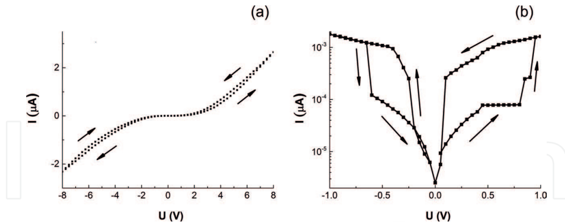
Figure 14. I-V characteristics of the Pt/GO/Pt structure after electron irradiation before (a) and after (b) the forming process.
