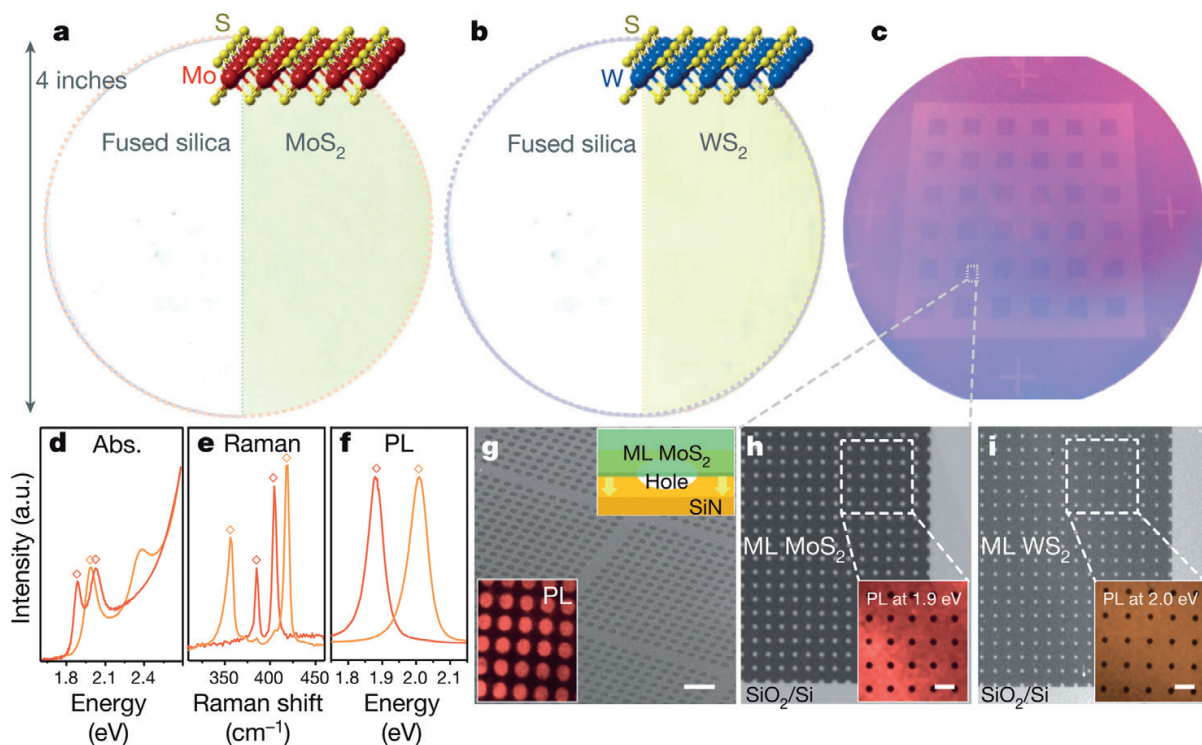
Figure 20. Single-layer transition metal dichalcogenides (TMD) films on 4-inch wafers. a, b, photos of MoS 2 (a) and WS 2 (b) monolayers of films grown on 4-inch substrates with diagrams of their respective atomic structures. The left halves show a quartz substrate for comparison. (c) Photo of a patterned monolayer MoS 2 film on a 4-inch SiO 2 /Si wafer (the darker areas are covered with MoS 2 ). (d) Optical absorption spectra of the MOCVD-grown monolayer MoS 2 (red line) and WS 2 (orange line) in the photon energy range from 1.6 to 2.7 eV. (e) The Raman spectra of the grown monolayer MoS 2 and WS 2 normalized to the intensity of the silicon peak. (f) Normalized photoluminescence spectra of monolayers MoS 2 and WS 2 grown. The peak positions in d–f are consistent with the positions of the peaks obtained from the peeled samples (diamonds). (g) SEM image and photoluminescence (PL) (bottom insert, at 1.9 eV) of monolayer (ML) MoS 2 membranes suspended on a SiN TEM mesh with holes of 2 μm (the suspended film scheme is shown in the upper inset). Label, 10 microns. (h), (i) Optical images (normalized to the area of a clean substrate) of the patterned monolayer MoS 2 (h) and WS 2 (i) on SiO 2 taken from films with a wafer-scale pattern. The insets show photoluminescent images for energies of 1.9 eV (h) and 2.0 eV (i). Scale mark, 10 microns [22].
