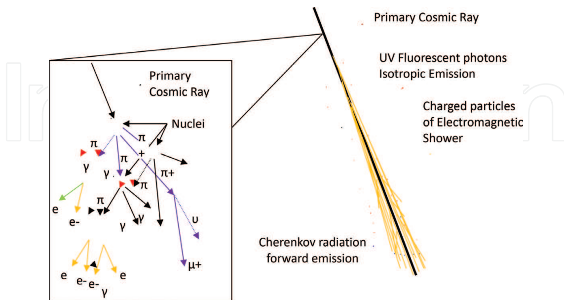
Figure 2. The schematic of the hadronic and electromagnetic components generation in the EAS development.
