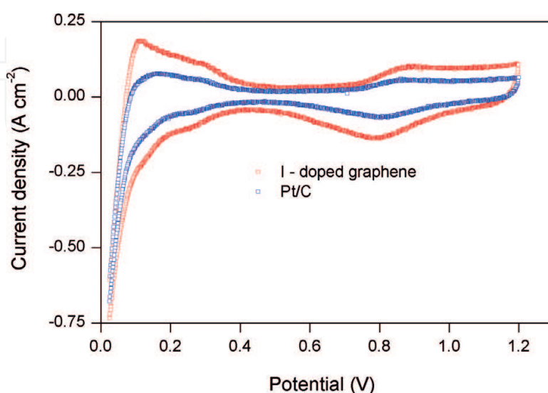
Figure 7. Cyclic voltammetry performed on in situ FC measurements in following operation conditions: temperature— 60^\circ\text{C} ; the air in the original FC cathode was replaced with \text{N}_2 ; potential scan rate— 50 \text{ mV/s} .
