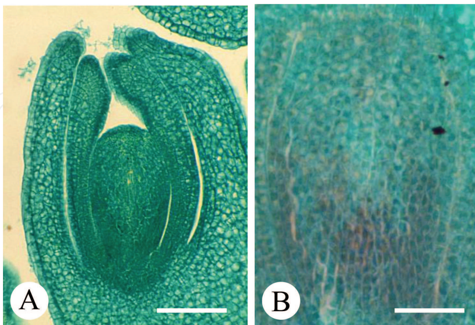
Figure 9. Ovule morphology and embryo sac development in the haploid pummelo [32]. A: Ovule morphology at 3/4 size of flower bud. Bar = 100 \mu\text{m} . B: No embryo sac at 2 days after flowering. Bar = 50 \mu\text{m} .
