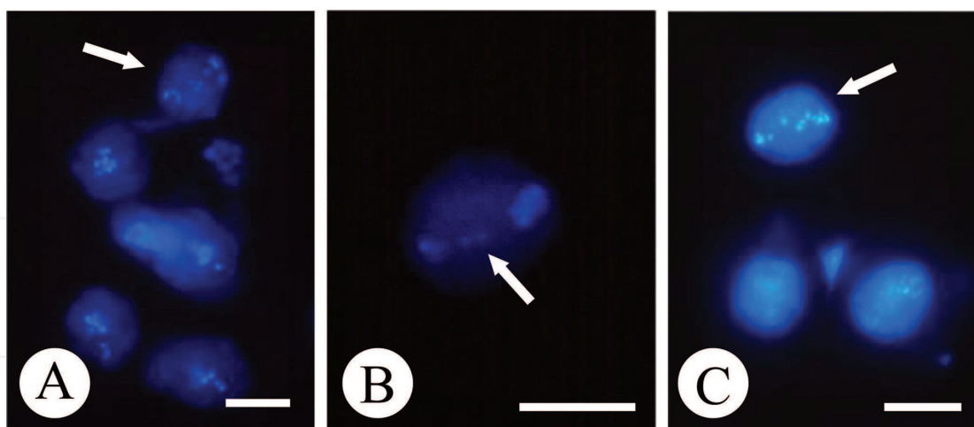
Figure 13. Abnormalities of the meiotic stage of the haploid pummelo [32]. A, B: Chromosomes remained in the equatorial plane, C: Nine bivalents aligned in the equatorial plane. Bars = 10 \mu\text{m} . Arrows indicate the abnormal cell.
