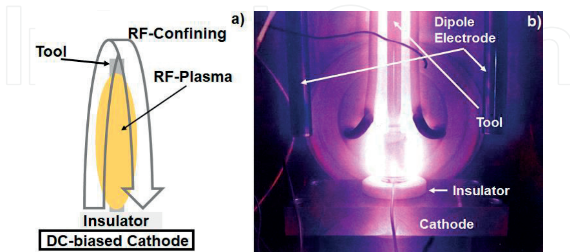
Figure 20. Down-sizing of an ashing unit for plasma oxidation of miniature parts and tools.
