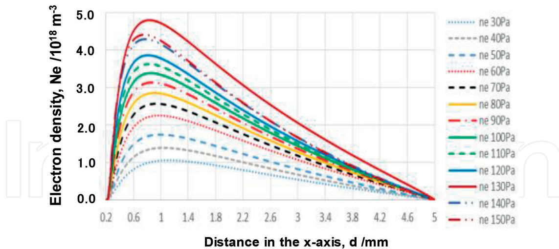
Figure 19. Enhancement of electron density distributions with increasing the argon pressure.
