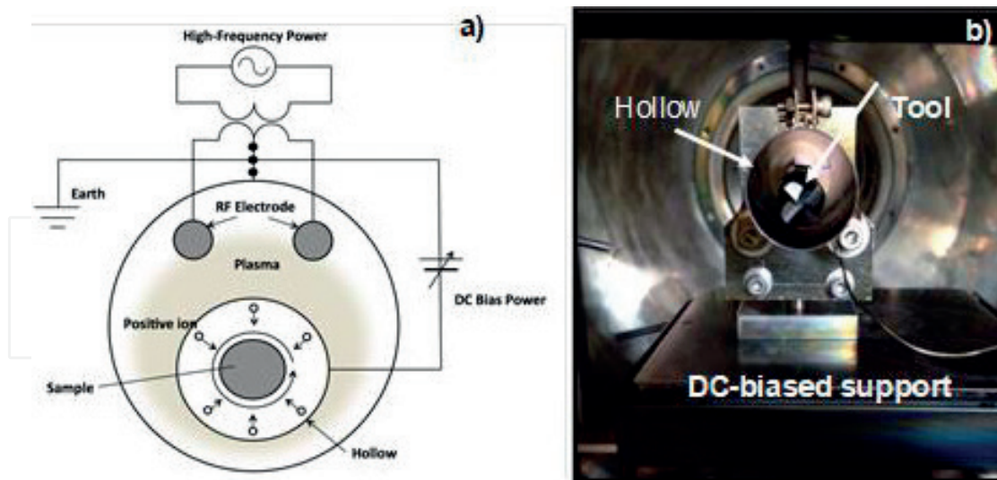
Figure 9. Special hollow cathode device for ashing the diamond films on the WC (Co) end-milling tool substrate. (a) Illustration of hollow cathode device, and, (b) experimental set-up for ashing.
