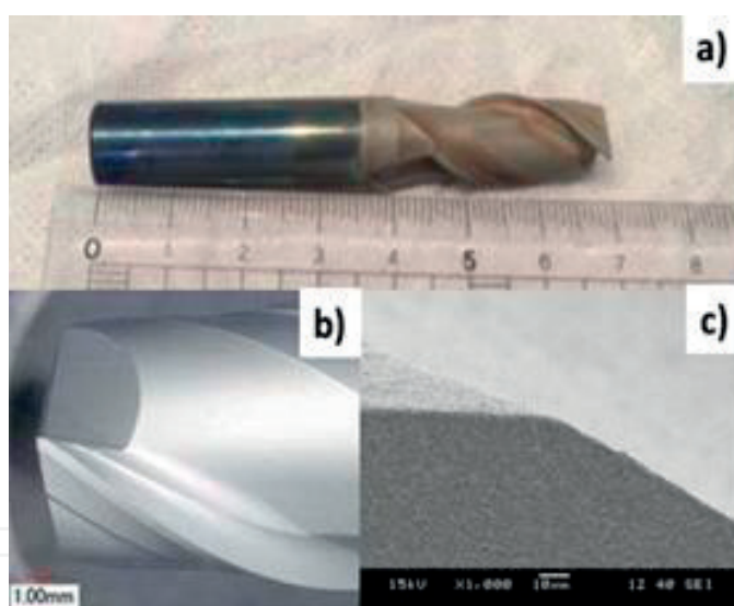
Figure 11. Ashing of CVD-diamond coating on the WC (Co) standard specimen under (250 V; -500 V; 45 Pa; 3.6 ks). (a) Surface of ashed specimen before cleansing, (b) Ashed tool edge, (c) SEM image of tool edge.
