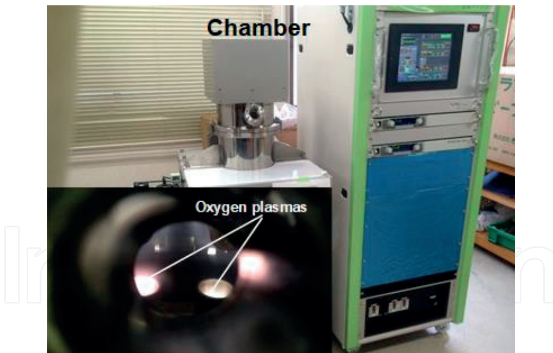
Figure 21. Simultaneous ashing system of two diamond-coated cutting tools toward industrial demonstration.
