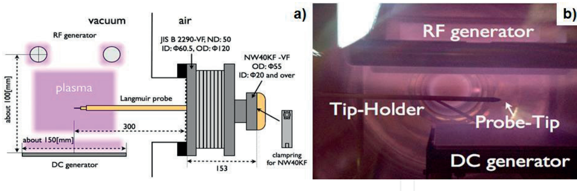
Figure 5. Experimental set-up for measurement of ion and electron densities as well as electron temperature at the specified position in the RF/DC plasmas by using the Langmuir probe.
