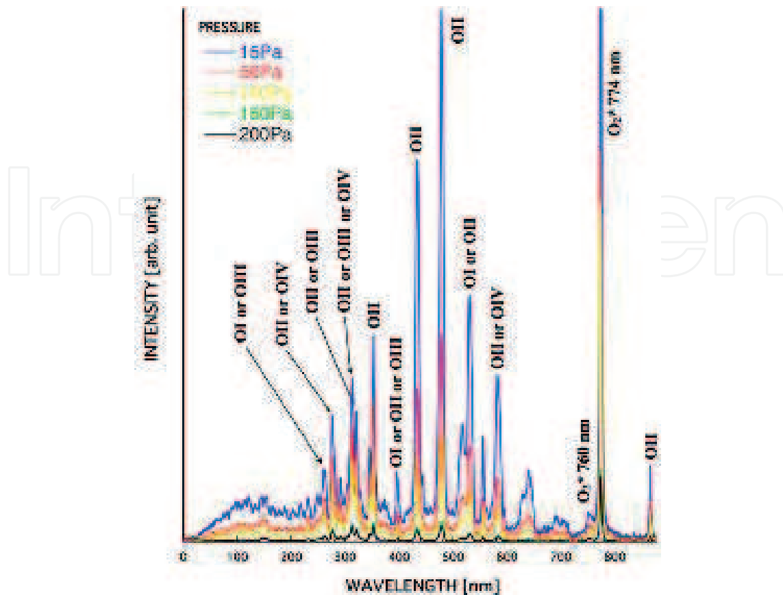
Figure 4. Measured emissive light optical spectra in the function of gas pressure for a standard RF/DC plasma under [250 V; -500 V].
