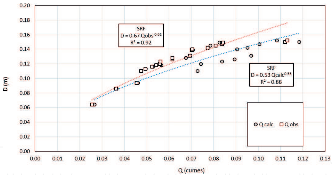
Figure 6. Observed data and calculated rating curves for smooth rectangular flow.
