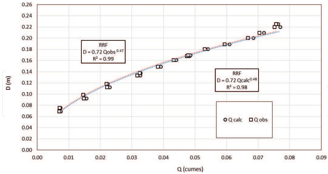
Figure 5. Observed data and calculated rating curves for roughness rectangular flow.
