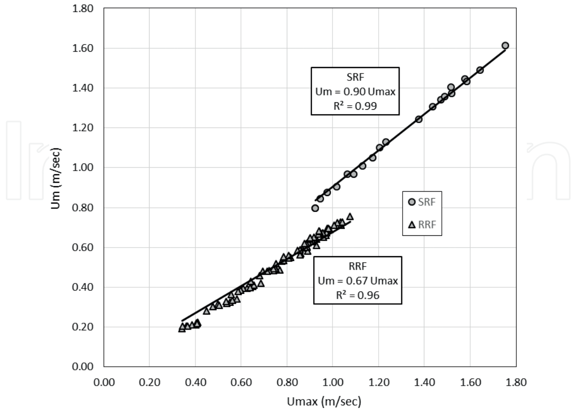
Figure 2. Average vs. maximum velocities observed for rough and smooth channel.
