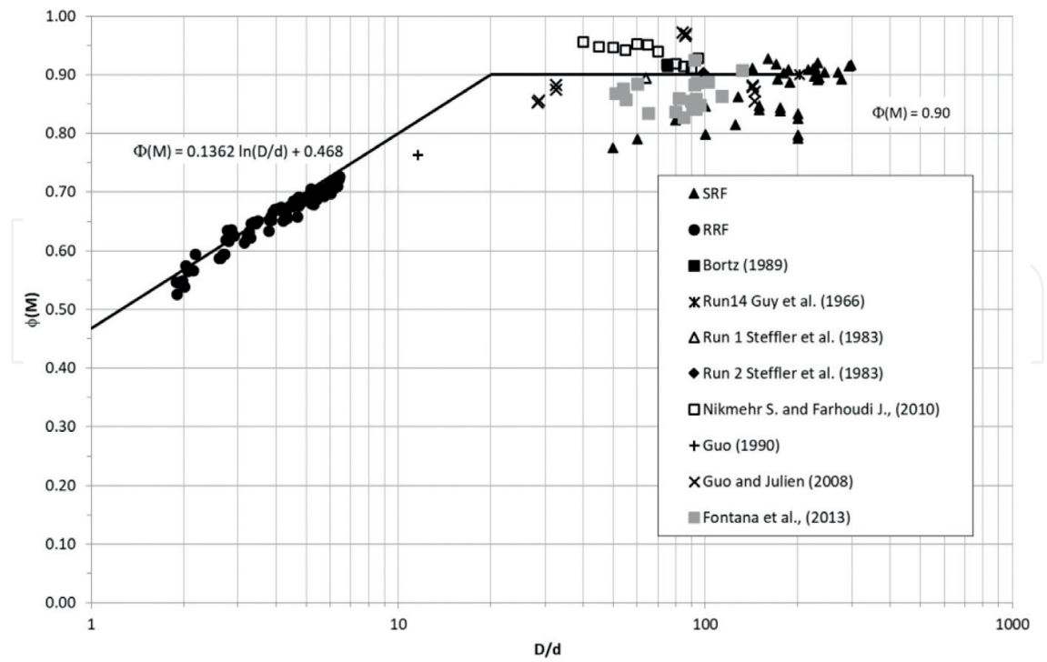
Figure 3. Velocity ratio vs. relative submergence.
