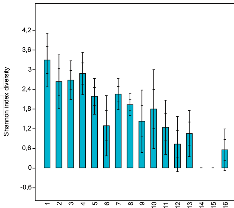
Figure 11. Box plot of the Shannon index.
