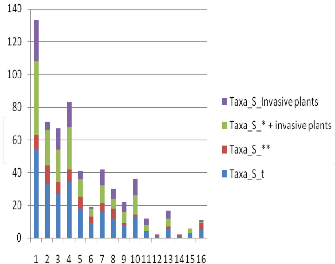
Figure 10. Graph showing the number of characteristic and invasive species.
