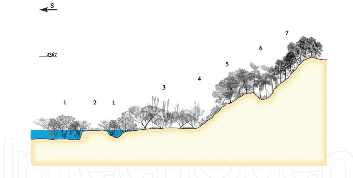
Figure 8. Profile of the vegetation of the cloud forest of Sierra Bahoruco. (1) Rhabdadenio biflori-Laguncularietum racemosae and Lonchocarpus pycnophylli-Conocarpetum erecti . (2) Salt marshes of Batidi-Salicornietea . (3) Lonchocarpus pycnophylli-Cylindropuntietum caribaeae . (4) Melocacto pedernalensis-Leptochloopsietum virgatae . (5) Broad-leaved forest. (6) and (7) Cloud forest of Prestoea montana .
