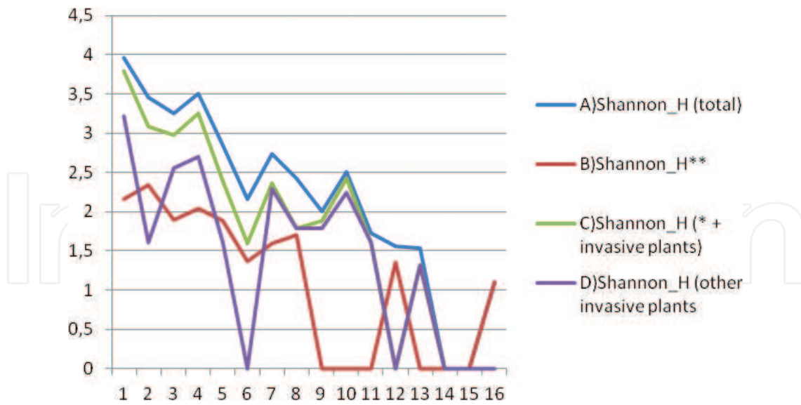
Figure 9. Shannon diversity graph of the four situations. (A) the total species in the community; (B) only characteristic mangrove species; (C) invasive species (both those growing in flooded areas, and invasive species due to the loss of the lake basin); (D) invasive species from nearby communities due to the silting of the lake basin.
