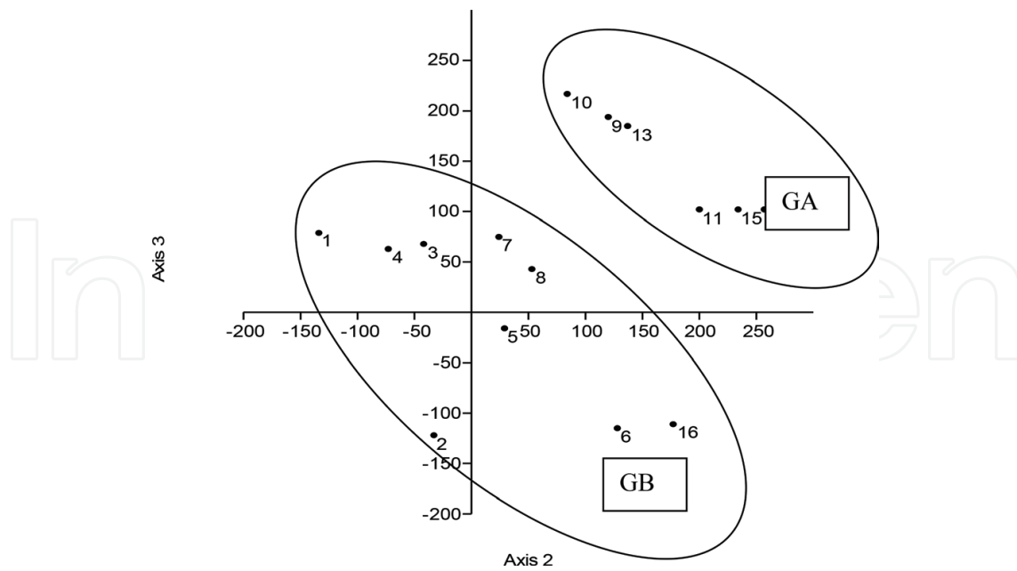
Figure 7. DCA ordination analysis separating the two groups (group GA and group GB) of mangrove communities.
