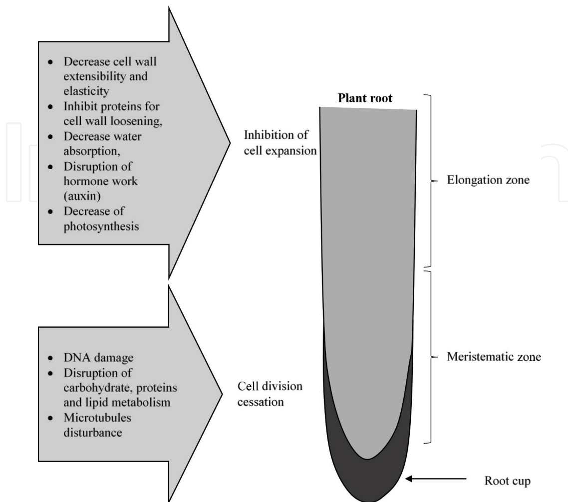
Figure 3. Effect of metal toxicity on roots cell growth involving multifaceted physiological inhibition and disruption including inhibition of cell division in meristematic tissues and inhibition of cell expansion. Cell division cessation may be caused by DNA damage, disruption of carbohydrate, protein and lipid metabolism, and microtubule disturbance. Inhibition of cell expansion could be caused by decrease of cell wall extensibility, inhibition of proteins that work in cell loosening, decrease water absorption, disruption of hormone work and decrease of photosynthesis.
