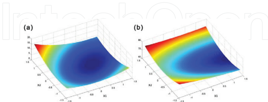
Figure 2. A 3D graphic of dependent factor (referring to final content of \gamma -cellulose Y ) vs. independent factors (referring to pressure X_1 and reaction time X_2 of the steam explosion process), (a) according to Eq. (5), and (b) according to Eq. (6).
