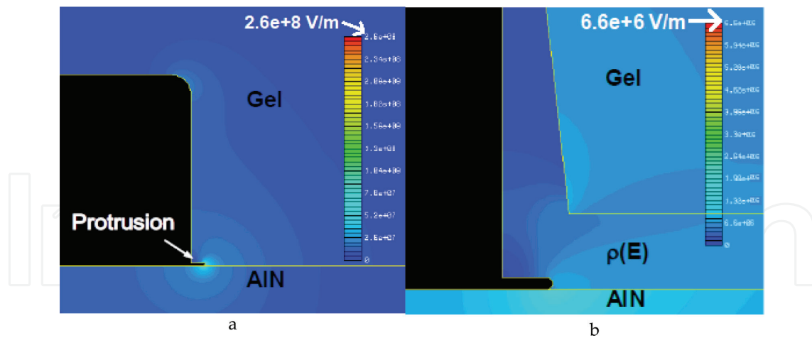
Figure 16. The influence of nonlinear FDC coating layer on reducing the electric field in the module [48], License No. 4383260855923.
