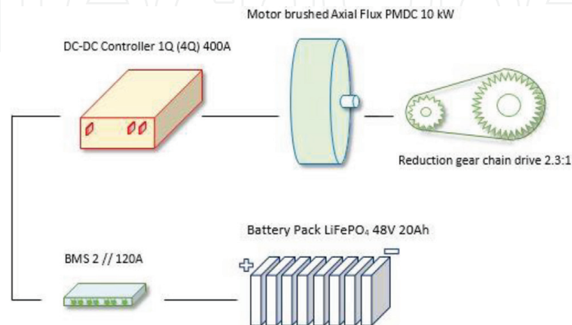
Figure 7. Final design summary.
