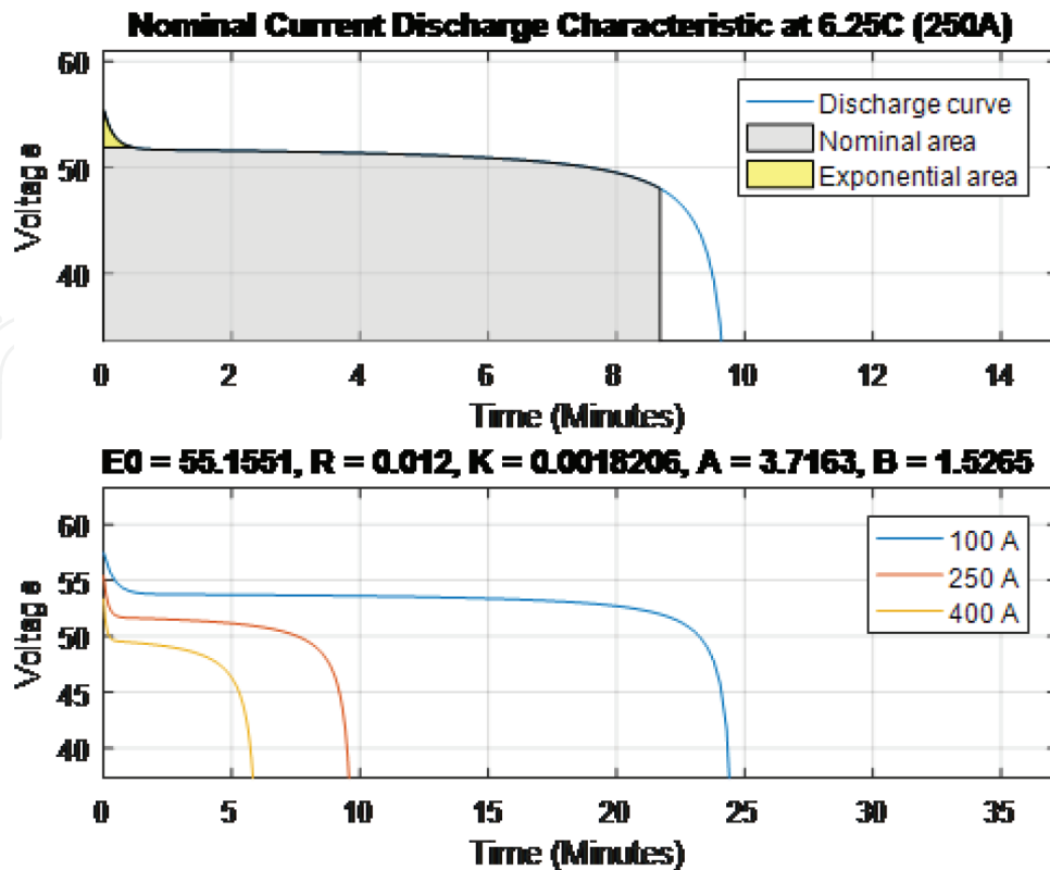
Figure 4. Battery discharge rates.
