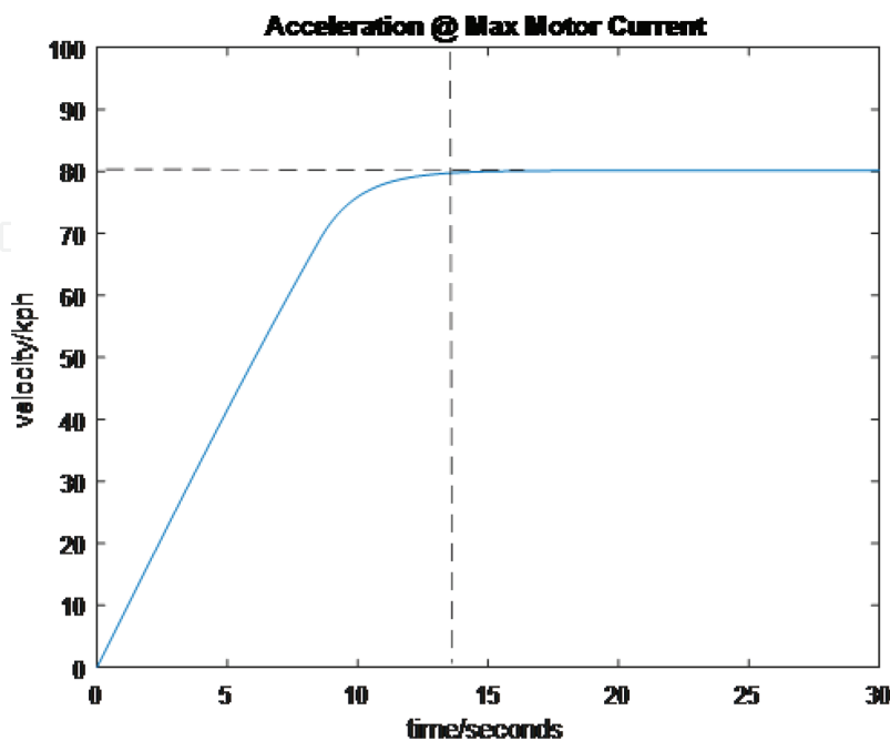
Figure 3. Vehicle acceleration under maximum load.
