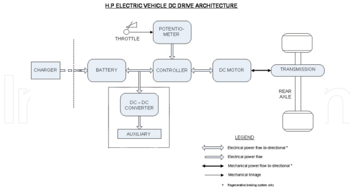
Figure 2. BEV DC drivetrain architecture.
