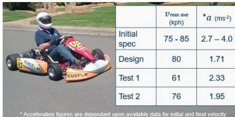
Figure 11. Vehicle performance test data.
