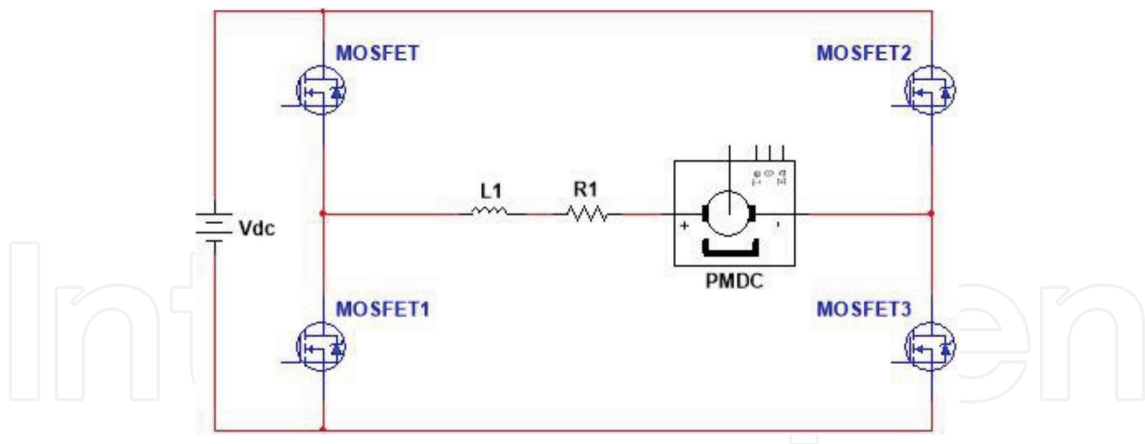
Figure 6. DC Q4 drive circuit.
