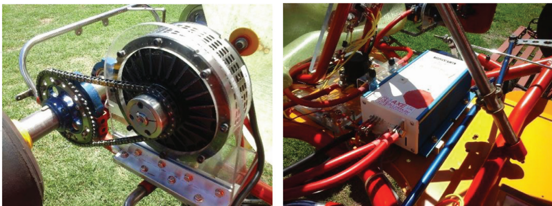
Figure 8. PMDC 10 kW motor and Q1 450 A controller.
