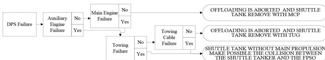
Figure 2. Event sequence diagram of the accident progression for offloading operation.
