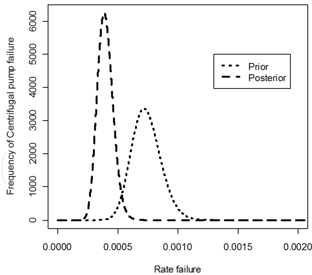
Figure 4. The prior density and posterior density for centrifugal pump failure rate.
