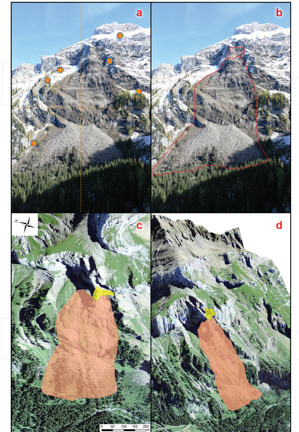
Figure 7. Spitzhorn rockslide (Gstaad, 2017). (a) Original oblique images with control points. (b) Digitalization of the detachment and transit/deposit zone on the original oblique image. (c) Projection of the digitalized contours on the current orthophoto. (d) Projection and 3D viewing of the digitalized zones in ESRI ArcScene. Yellow contours = detachment zone; orange contours = transit and deposit zone.
