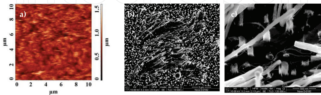
Figure 2. The images of the VA CNT array obtained after scanning in a semi-contact mode with a pressing force of the AFM probe to surface more than 10 \mu\text{N} : (a) AFM images; (b) and (c) SEM images.
