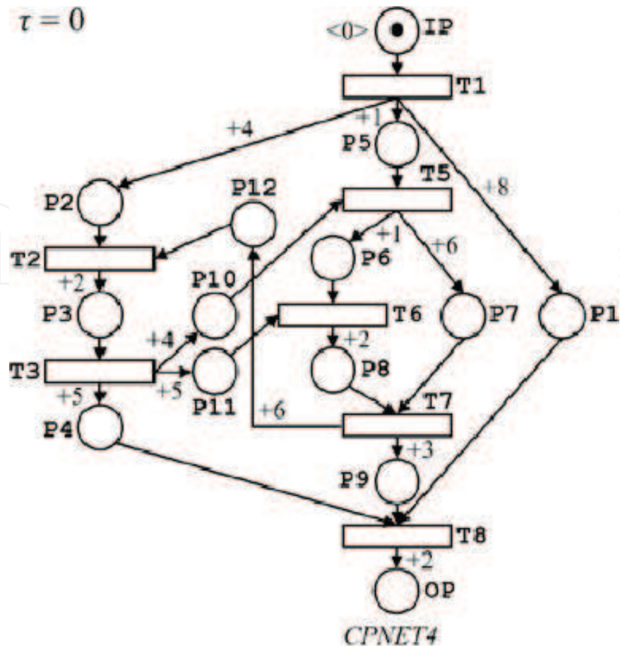
Figure 6. PNTS CPNET4 in its entry state S_e .
