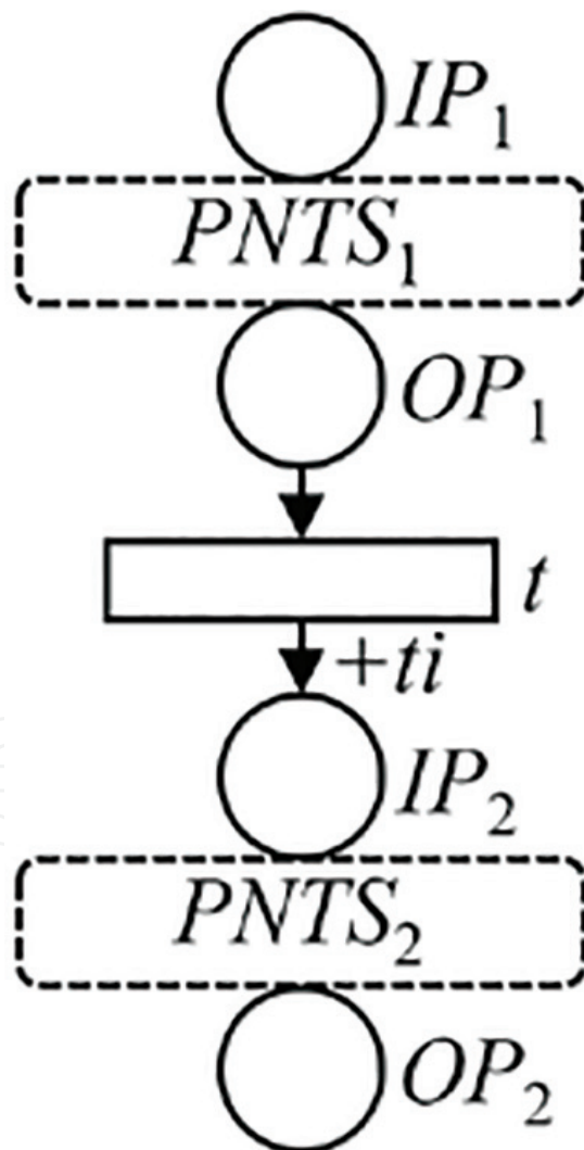
Figure 2. Symbolic representation of PNTS [PNTS_1, PNTS_2].COMP(t, ti) .
