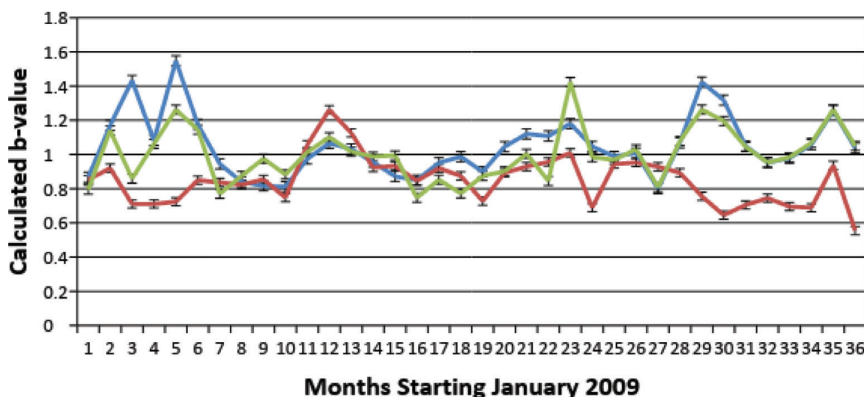
Figure 1. Continuous monthly b -variations as calculated by [14] from the seismicity data of NEIC (blue), ISC (red), and IRIS (green) that occurred during the period 2009–2011 with M \geq 4.5 . Bars represent the calculated standard errors.
