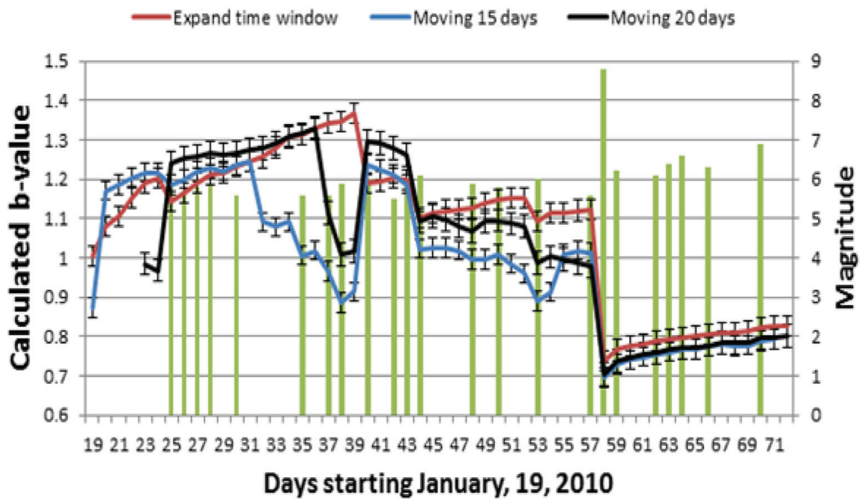
Figure 4. Variation of the b -values in Quadrant 3 of the Earth during a period of 39 days before and 14 days after the Chile, 2010, earthquake ( M_w = 8.8 ) as calculated by [14].
