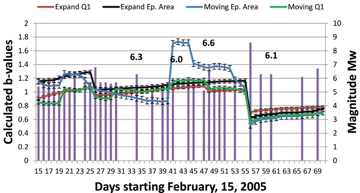
Figure 6. The b -variations as calculated by [14] for Quadrant 1 (red) and the epicentral area (black) of the Sumatra 2005 M_w = 8.6 utilizing daily expanding time windows. The first window expands between Feb. 8 and Feb. 15, while the last expands between Feb. 8 and April 11, 2005. The green and blue curves represent the calculated b -values for both regions utilizing a 15-day window that moves 1 day at a time. All epicentral earthquakes M \geq 5 are marked. Only four earthquakes ( M_w \geq 6 ) occurred outside Sumatra epicentral region but within Quadrant 1 are marked with their magnitudes.
