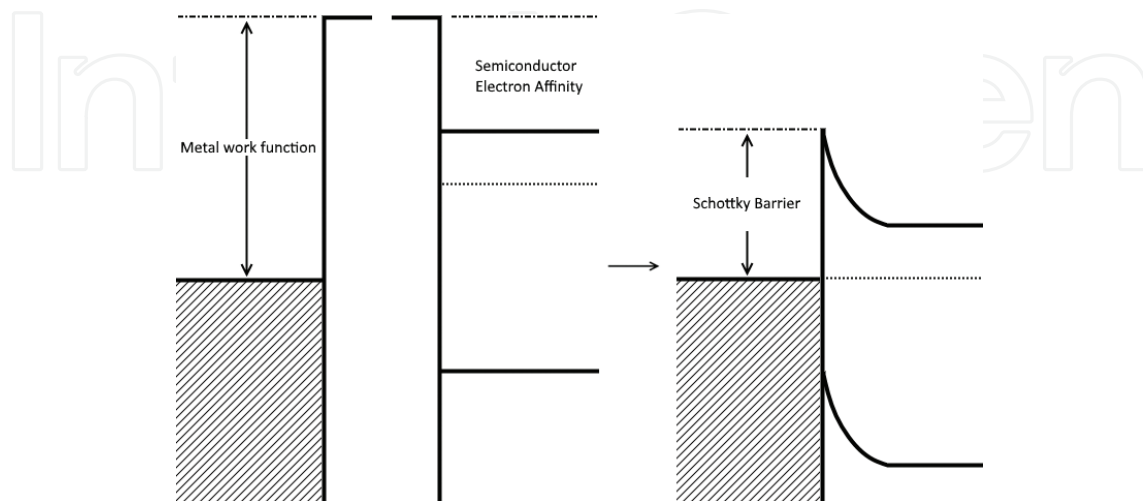
Figure 1. Band structure of Schottky barrier formation [1].
