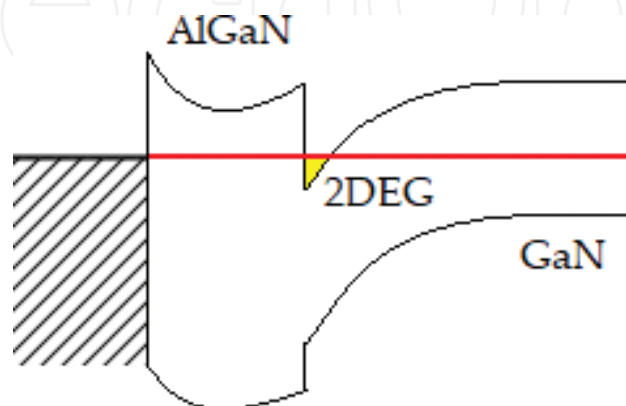
Figure 5. Band structure of the AlGaIn/GaN heterostructure.
