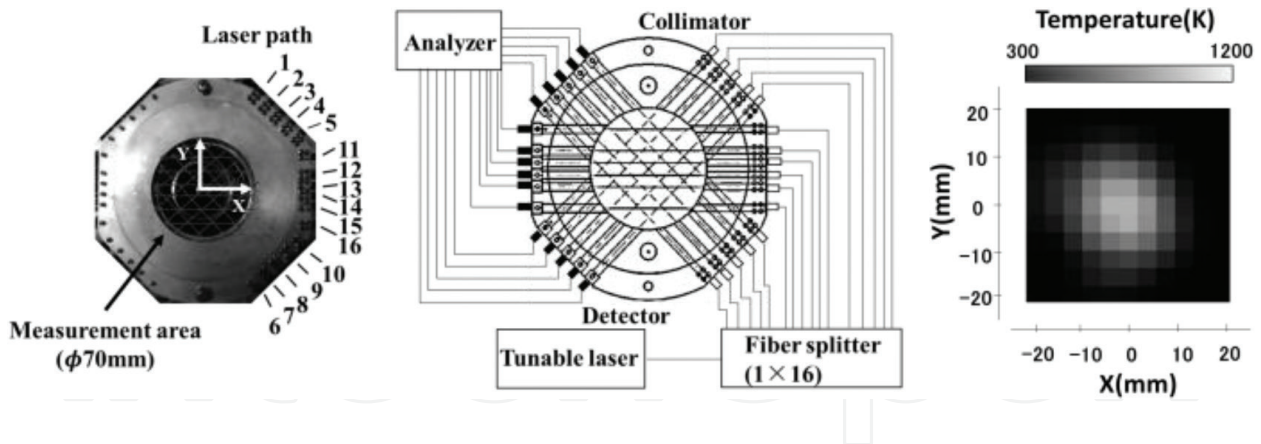
Figure 10. CT measurement cell and temperature measurement result [10].
