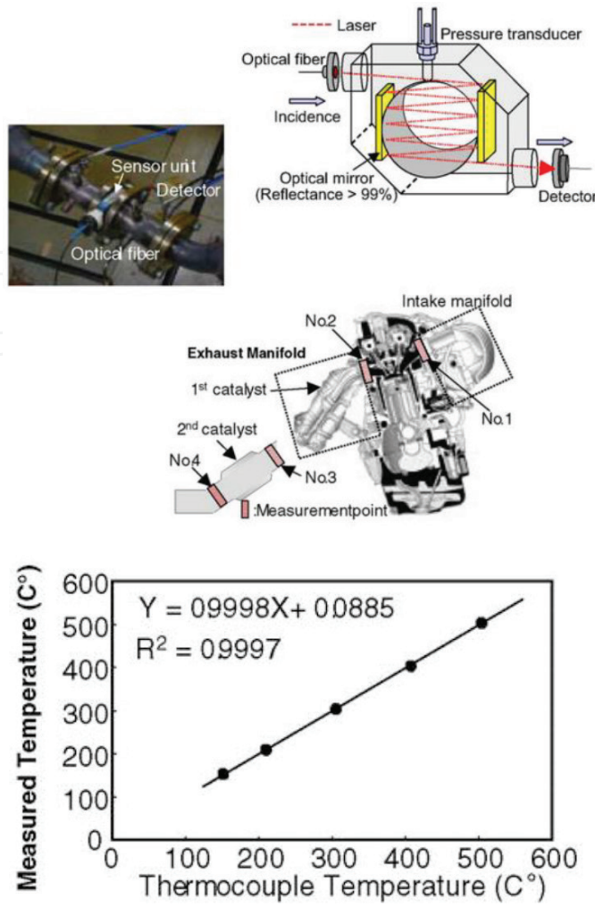
Figure 7. Application of TDLAS to engine exhausts and intake air measurements. (a) Measurement positions and schematic of sensor unit. (b) Temperature measurement result [22].
