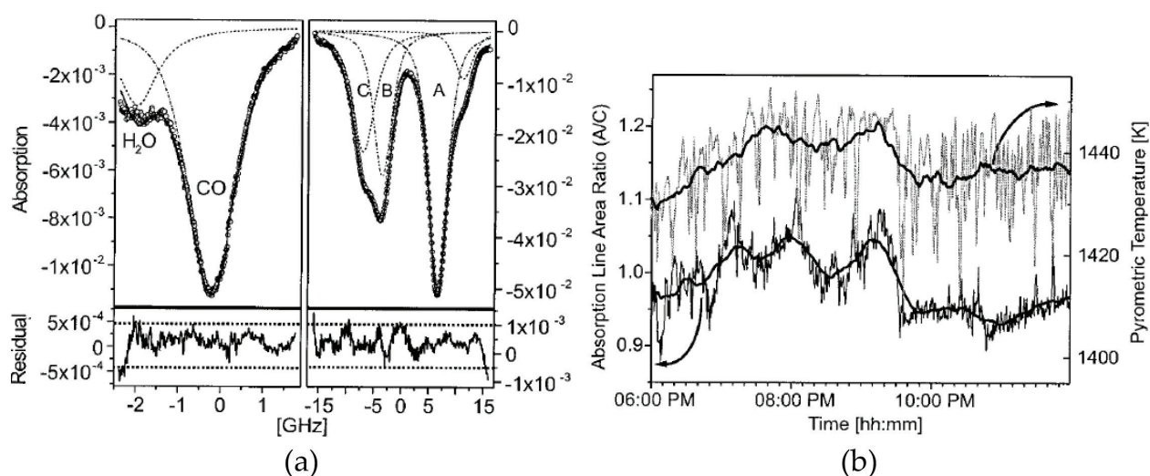
Figure 15. Measurement results of spectra and temperature. (a) Typical in situ line shapes of CO line at 1559.5 nm and H_2O at 813 nm. (b) Time series of the line area ratio of H_2O lines compared with temperature data from the radiative pyrometer [37].
