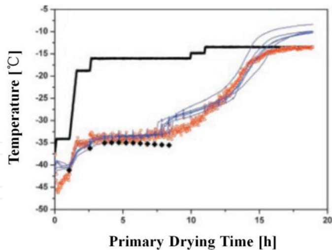
Figure 16. TDLAS product temperature calculation during a SMART freeze dryer run processing 5% (w/w) sucrose (3 mL fill volume/vial, 112 vials total load, 20 mL Wheaton). Symbols represent thick solid line = shelf inlet temperature, empty circles = T_{p-TDLAS} , thin solid lines = T_{b-TC/center} ( n = 5 ), filled diamonds = T_{p-MTM} [44].
