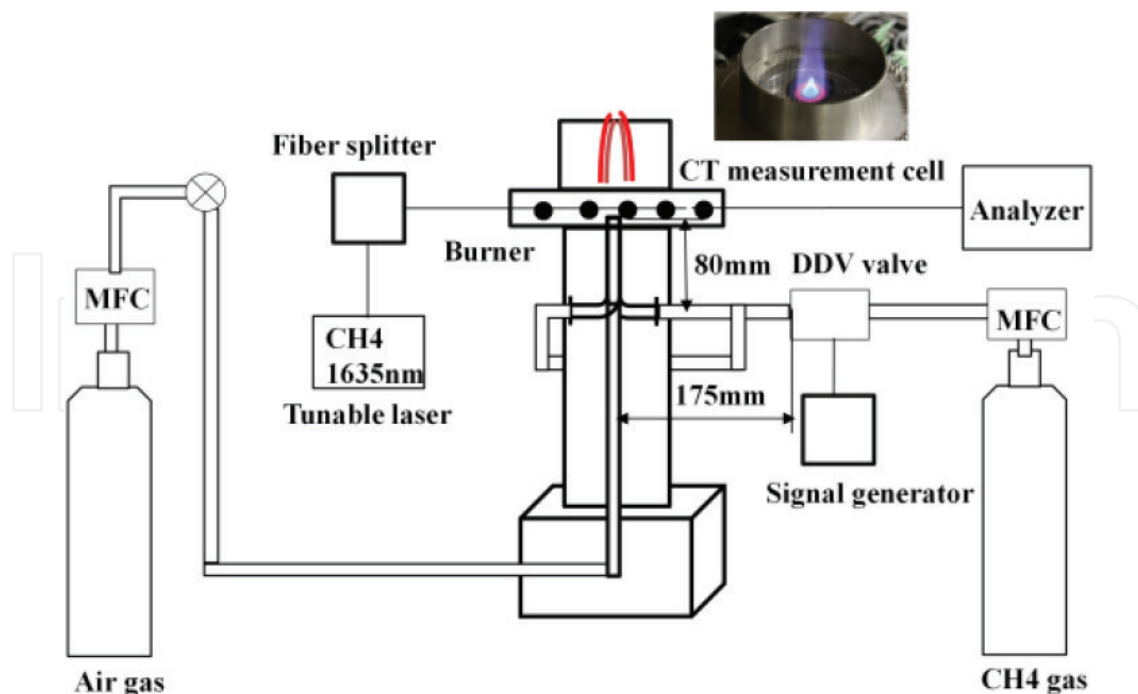
Figure 13. Experimental setup of time-resolved 2D temperature and \text{CH}_4 concentration in an oscillating \text{CH}_4 -air Bunsen-type flame using CT-TDLAS [11].
