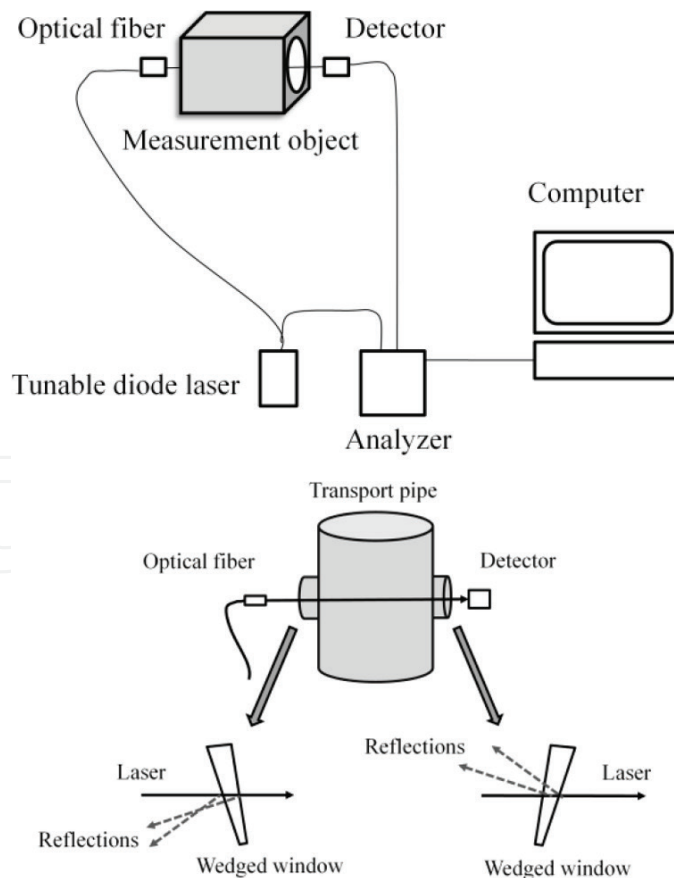
Figure 6. Typical geometric arrangement of TDLAS. (a) Typical geometric arrangement. (b) Wedged windows used in the laser pass.
