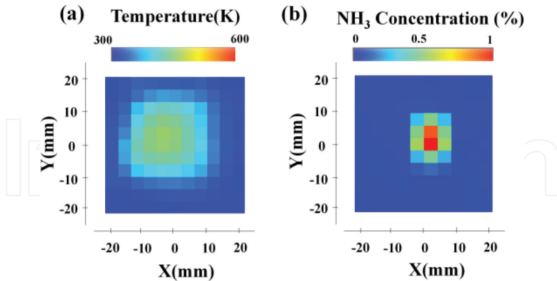
Figure 14. 2D temperature and NH 3 concentration measured by CT-TDLAS [11].
