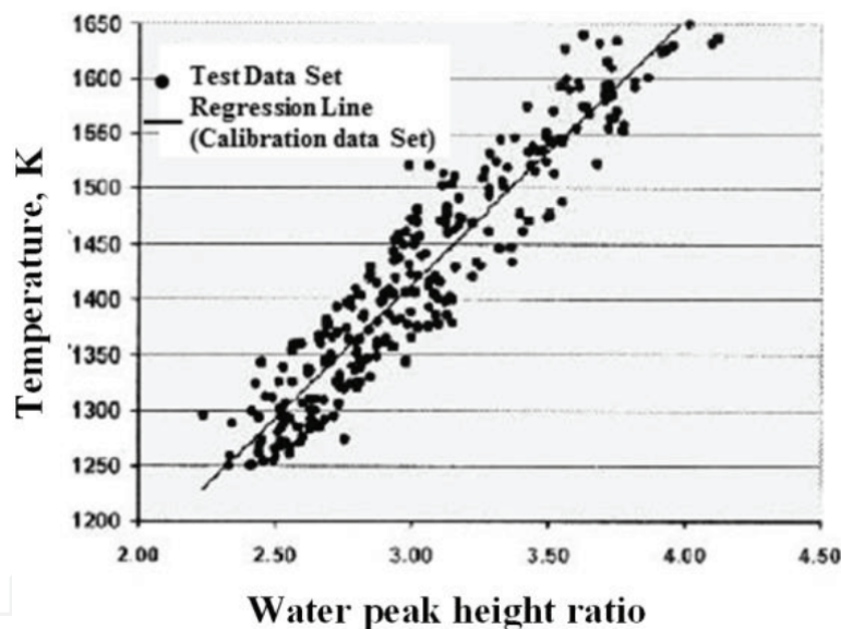
Figure 17. Comparison of the water peak height ratio with the thermocouple measurements [46].
