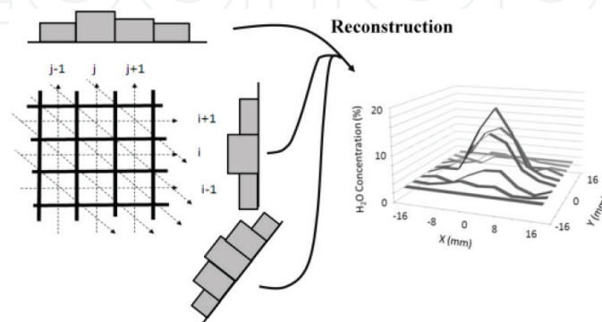
Figure 4. 2D image reconstruction by a set of absorption signals using CT.
