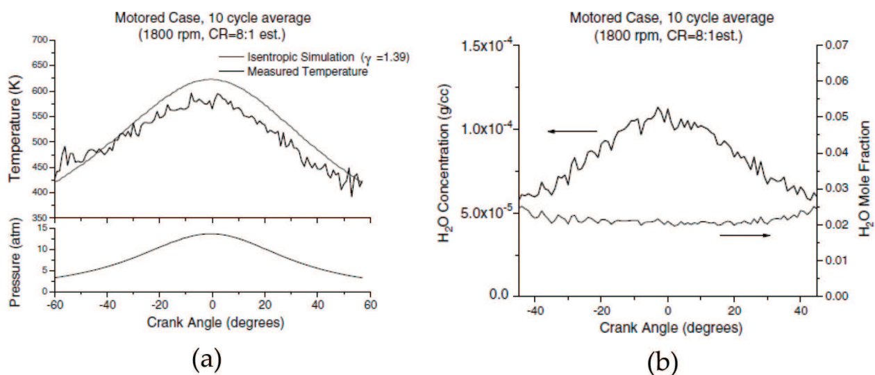
Figure 9. Gas temperature and H 2 O concentration measurement in a motoring, single-cylinder engine. (a) Measured temperature. (b) Measured H 2 O concentration [26].
