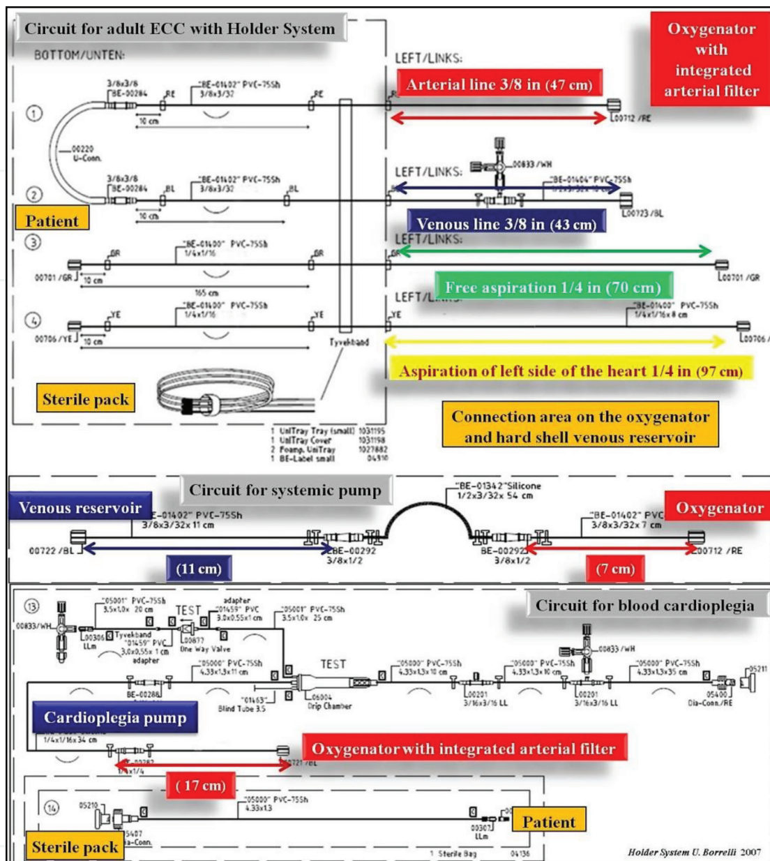
Figure 14. ECC circuit for adult patients with the holder system.
