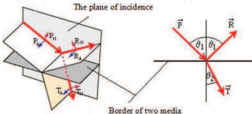
Figure 8. The EM wave reflection and transmission phenomenon.
