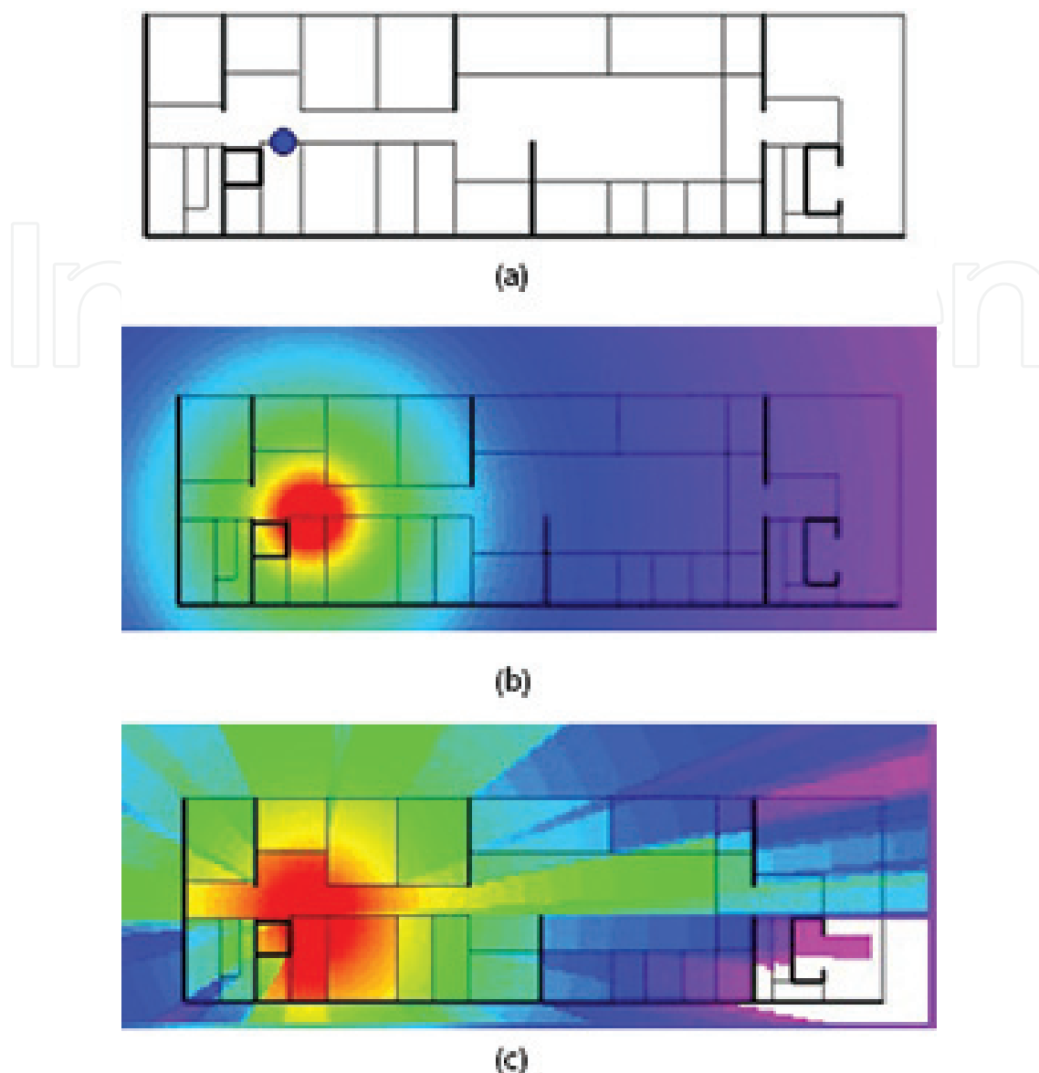
Figure 2. The projection of floors and location of the access point (a), the distribution of the signal for one-slope model (b), and for nonlinear model of multi-walls (c) [3].
