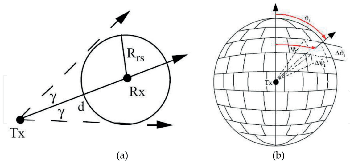
Figure 6. Cross-section of the receiving sphere (a) and rays launching method concept (b) [11].
