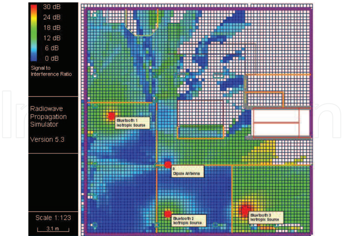
Figure 15. Levels of interference between Bluetooth and IEEE 802.11 g systems on the ground floor of the C-5 building.
