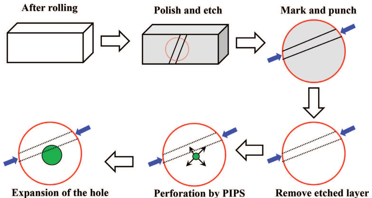
Figure 1. Schematic illustration of the preparation process for the TEM samples.
