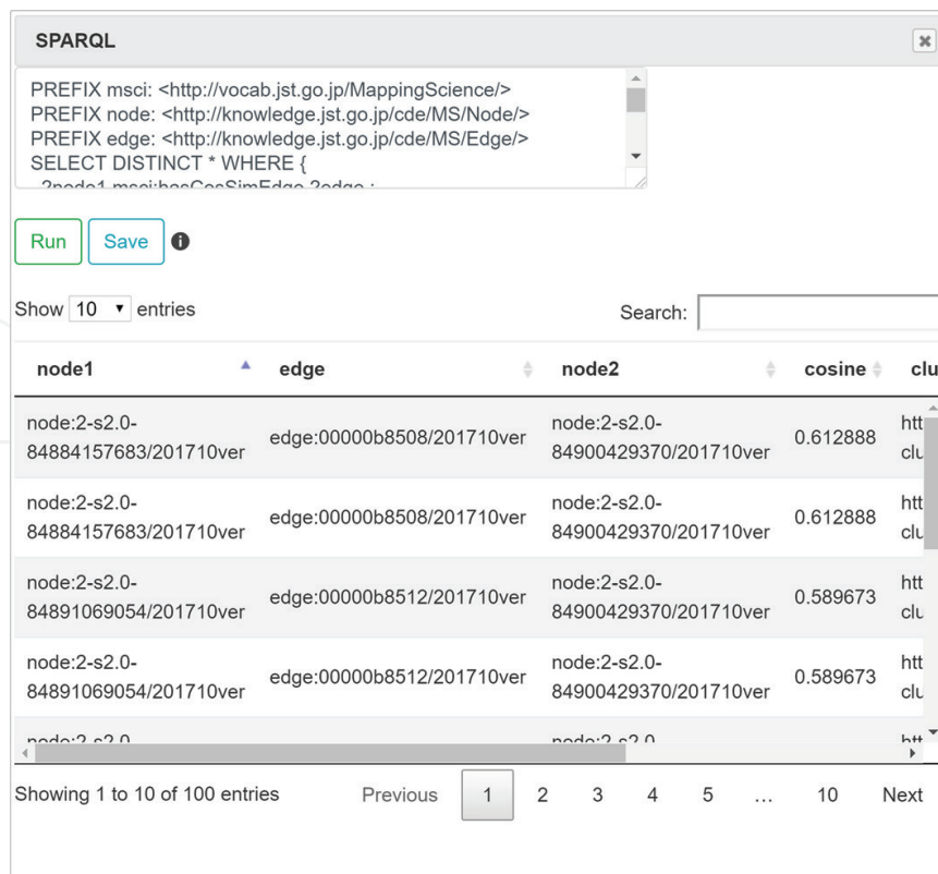
Figure 9. SPARQL search widget.
