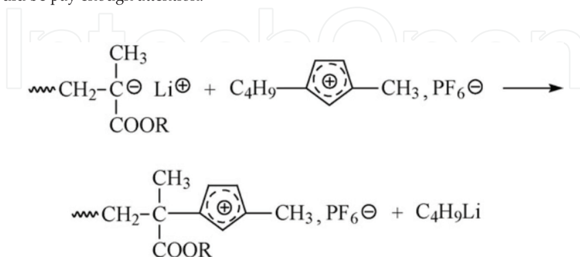
Figure 7. Chain transfer to ionic liquid in anionic polymerization of methyl methacrylate.
