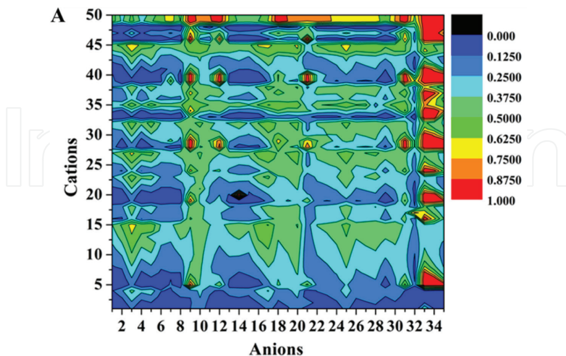
Figure 1. Predicted solubilities of p -methylstyrene in 1750 types (50 cations \times 35 anions) of ionic liquids.
