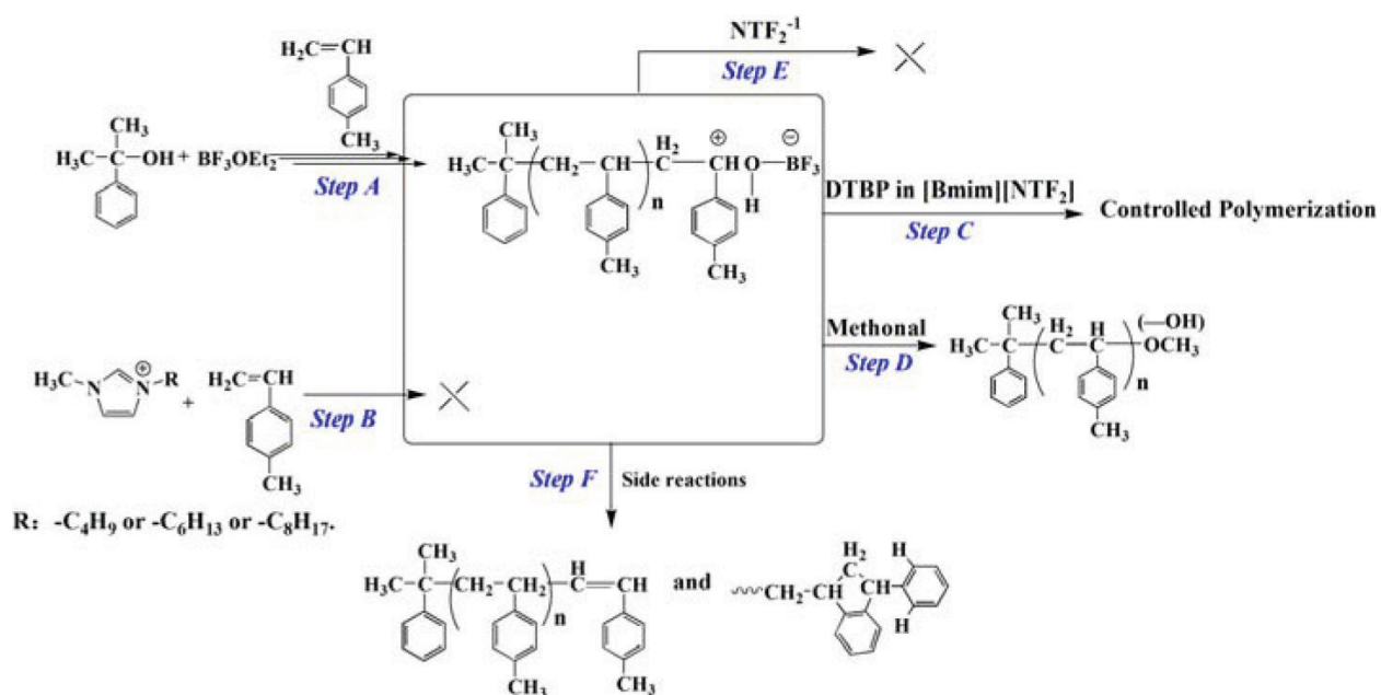
Figure 4. Proposed mechanism for the cationic polymerization of p -methylstyrene with the CumOH/ \text{BF}_3\text{OEt}_2 initiating system in \text{NTf}_2^{-1} based ionic liquids.
