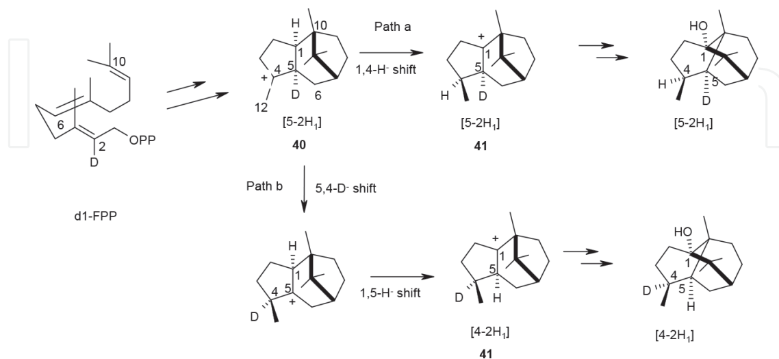
Scheme 15. Biosynthetic pathways for the conversion of [2-2H 1 ]-FPP to patchouliol isotopomer.
