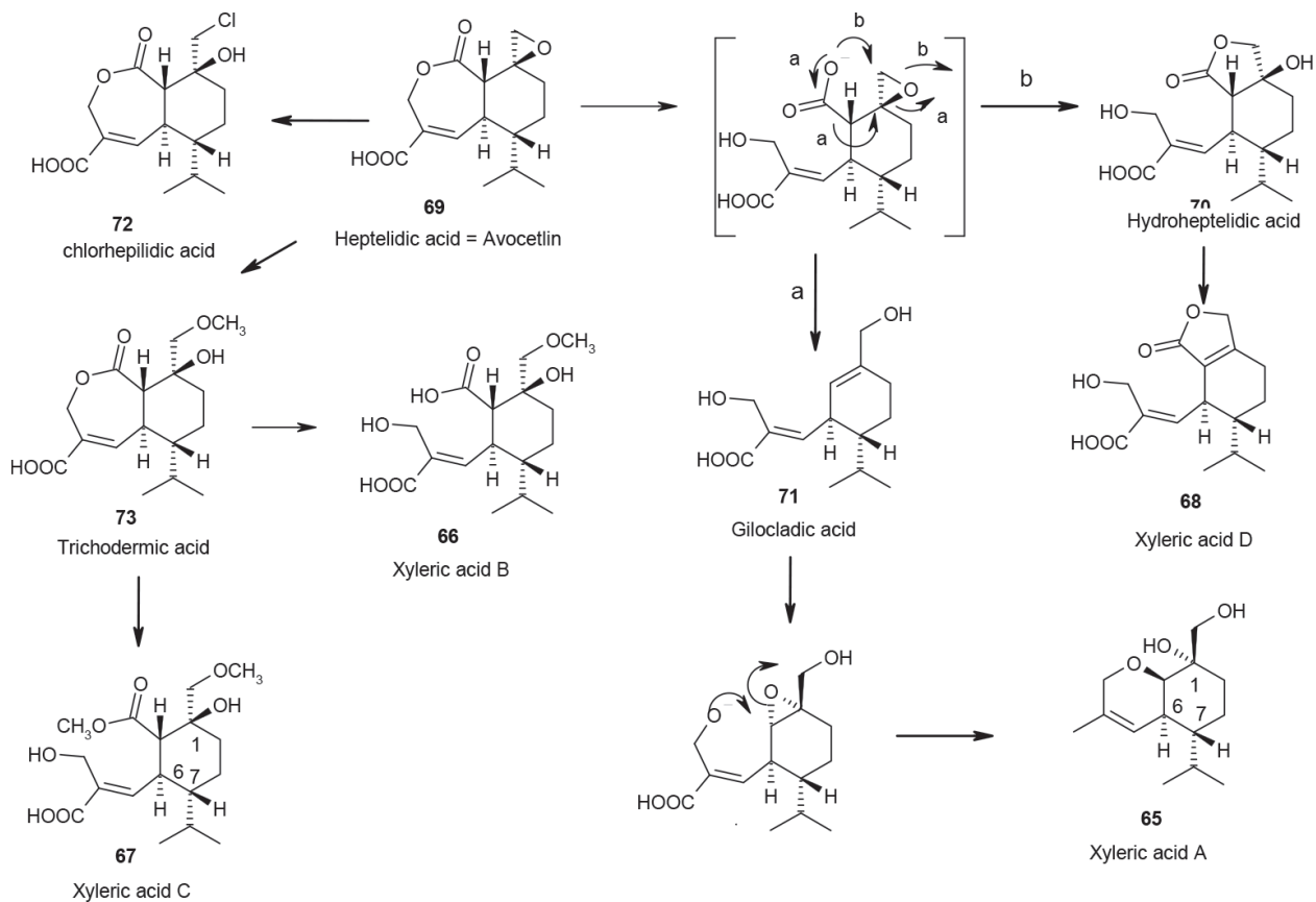
Figure 8. Structural interrelations among the congeners of Xylaria sp. and the sequence of formation of isolated metabolites 65–73.
