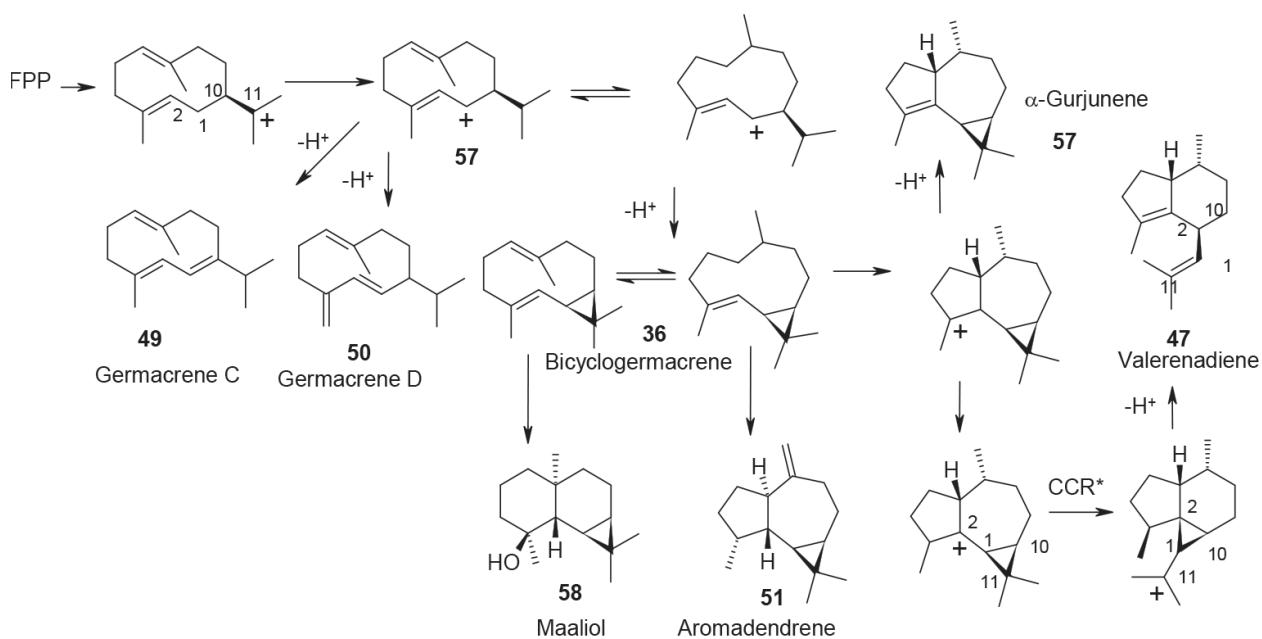
Scheme 19. A cyclopropane route to valerenediene 47 (numbering based on FPP).
