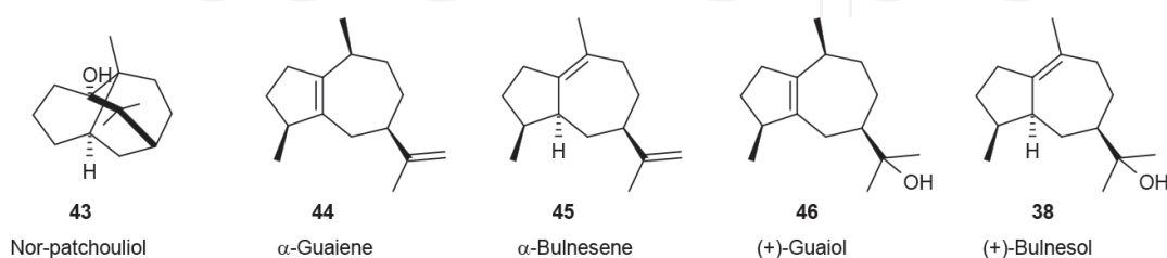
Figure 7. Structures of nor-patchouliol 43 , \alpha -guaiene 44 , \alpha -bulnesene 45 , (+)-guaiaol 46 and (+)-bulnesol 38 .
