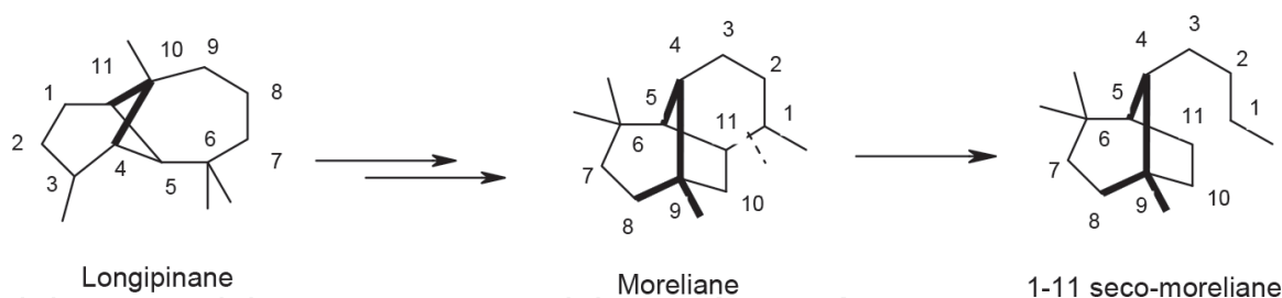
Figure 1. Skeletons of longipinane, moreliane and 1-11 seco-moreliane.
