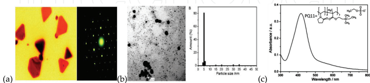
Figure 11. (a) Polygonal (mainly triangular) silver nanoprisms were synthesized by boiling AgNO 3 in N, N -dimethyl formamide and PVP, [88] (b) TEM image of as-formed silver colloids and the corresponding particle size distribution histogram and (c) UV-Vis spectrum of 150-fold diluted PQ-11 supported Ag NP solution of the dispersion synthesized at 100°C and 60min [89].
