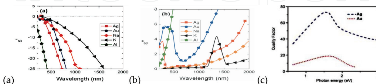
Figure 4. (a) Real and (b) imaginary part of permittivities of the metal candidates Ag, Au, Na, K, and Al [36]. (c) Quality factor of plasmon resonances of a metal nanostructure as a function of plasmon frequency for two commonly used metals: silver (dashed line) and gold (dotted line) [37].
