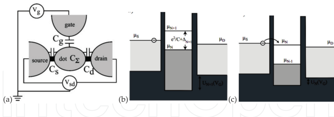
Figure 2. (a) Schematic diagram of typical arrangement of electrodes (quantum dot (QD) surrounded with source, drain and gate) for a single electron transistor. Energy diagram for a quantum dot, where the two tunnel barriers connected the QD to the source and drain contacts. (b) Electron transport is blocked and the dot contains a fixed number of N electrons. (b) Number of electrons on the QD can vary between N and N-1 , result in rise a peak in the conductance because the gate voltage was tuned in order to align the chemical potential of the QD with that of source and drain [15].
