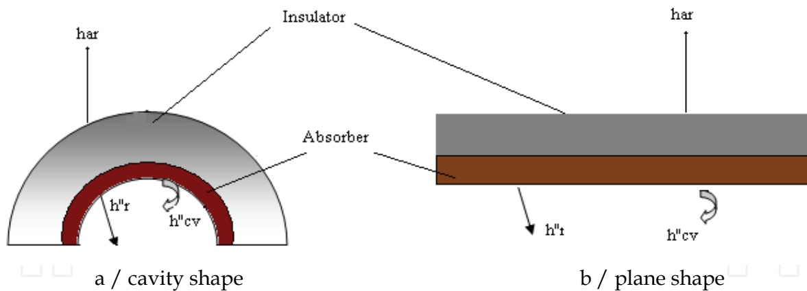
Fig. 13. Unprotected absorber.
