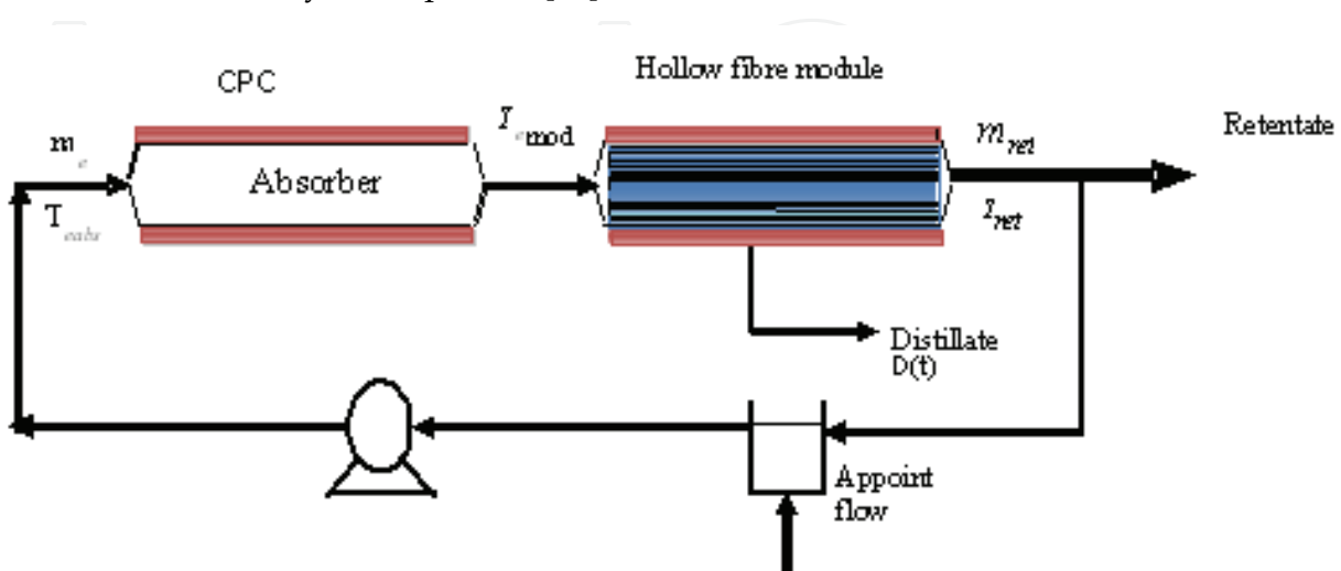
Fig. 10. Diagram of the desalination unit
