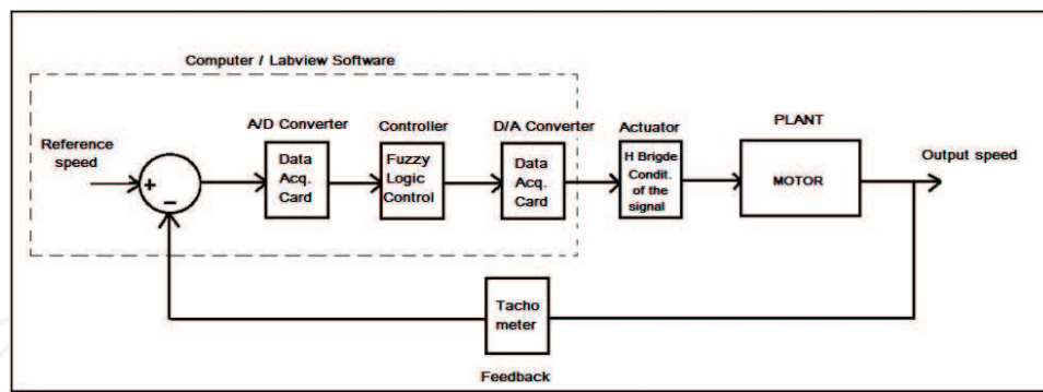
Figure 2. Process control (closed loop).
