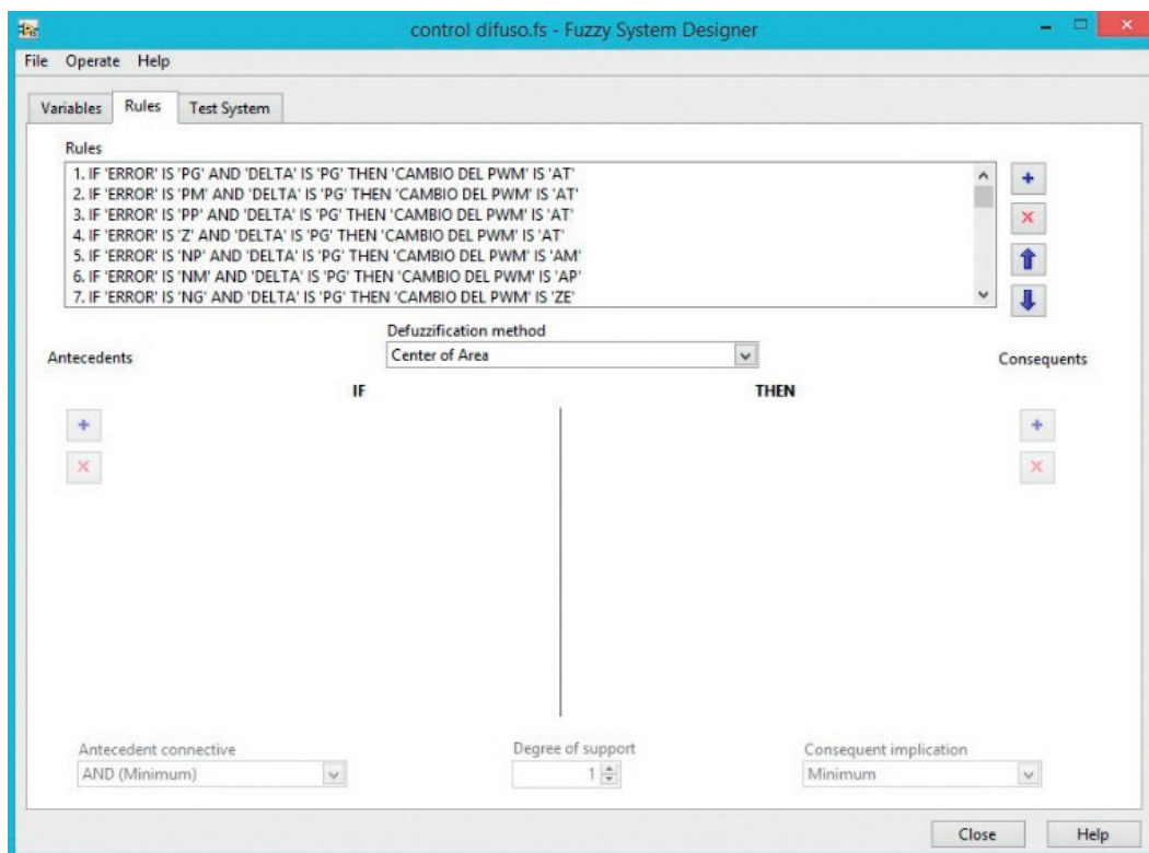
Figure 10. Rule editor.
