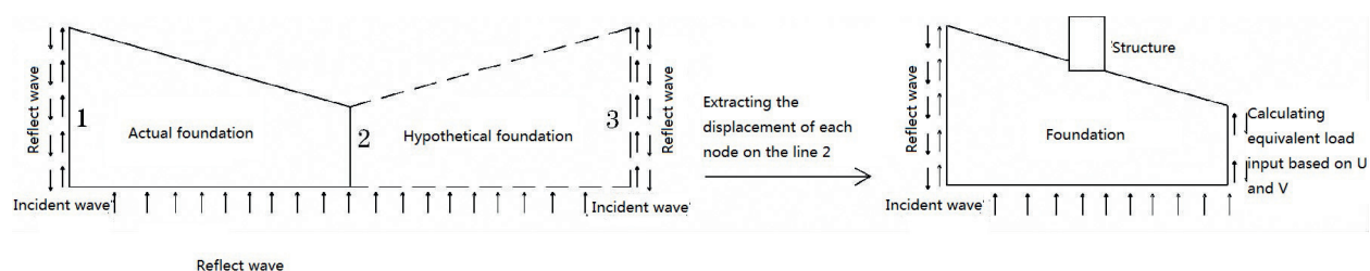
Figure 8. Sketch of recommended seismic input mode.
