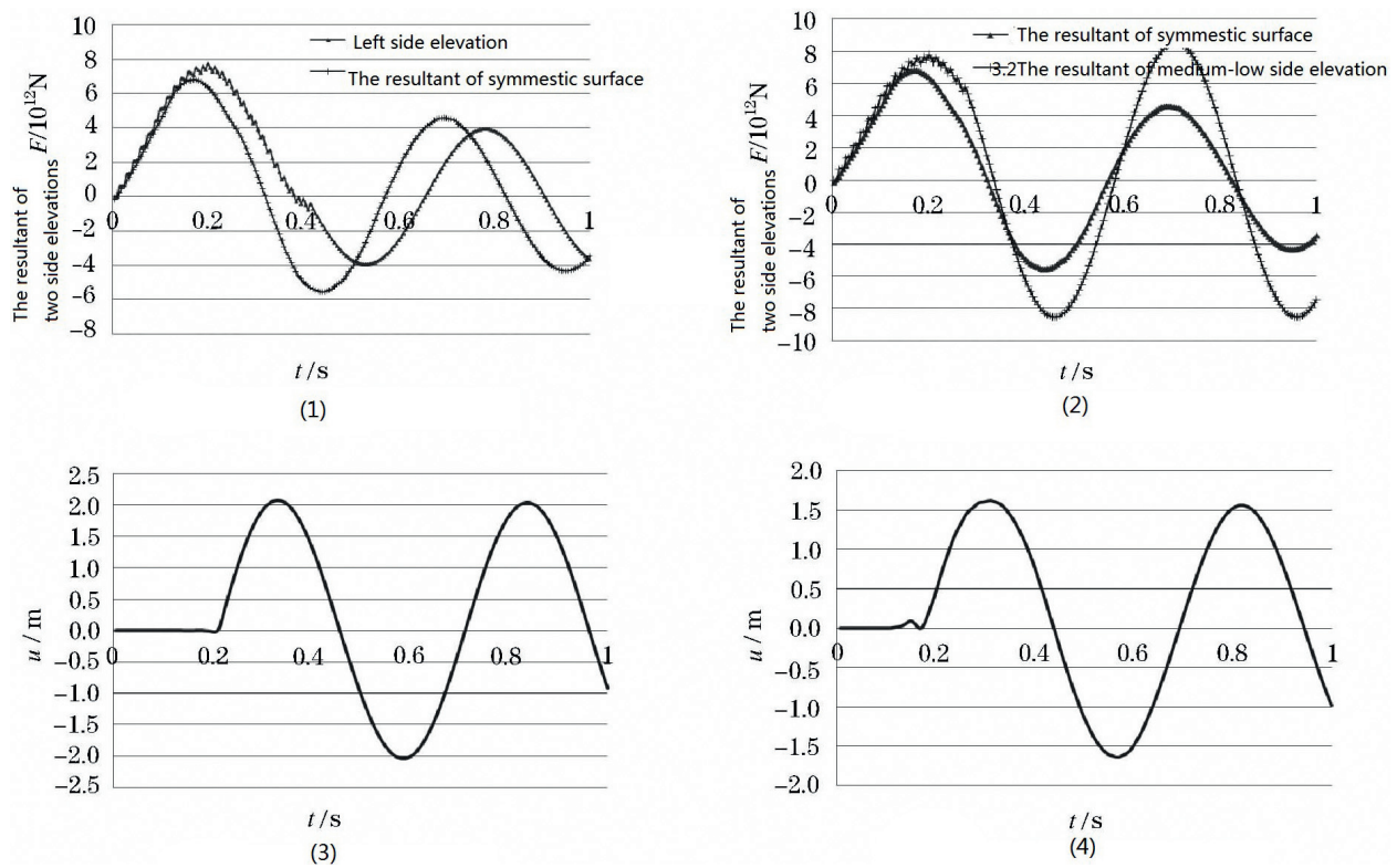
Figure 14. Dynamic response of symmetrical model. (1) Resultant force contrast between symmetry plane and left side elevation. (2) Resultant force contrast between symmetry plane and low side elevation. (3) Displacement time history of the vertex of left side elevation. (4) Displacement time history of the point with the height of 250 m.
