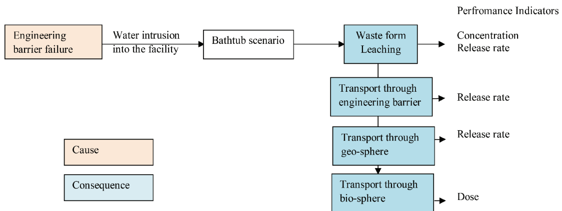
Figure 5. Conceptual model of disposal facility in a bathtub scenario.
