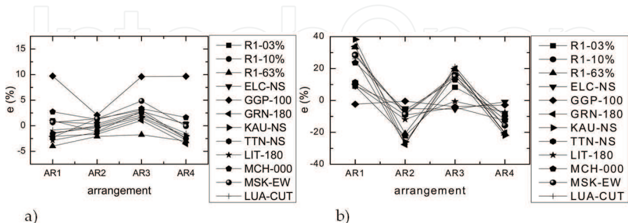
Figure 17. Interaction between surface structure and underground structure in terms of influence coefficient e for different arrangements under S waves producing motions along longitudinal axis ( d = 0.5 ), a) the impact on surface structure, b) the impact on underground structure.
