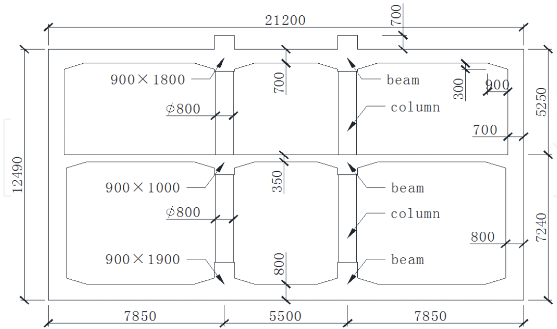
Figure 2. Cross-section of underground station (unit: Mm).
