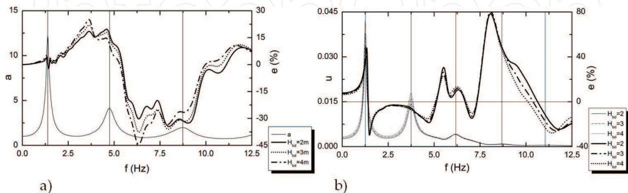
Figure 14. Interaction between surface structure and underground structure in terms of harmonic response spectra and influence coefficient e for different burial depth of underground station under S waves producing motions on the Y axis ( d = 0.5 ), a) the impact on surface structure, b) the impact on underground structure.
