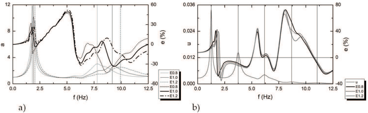
Figure 12. Interaction between surface structure and underground structure, arranged according to AR1, in terms of harmonic response spectra and influence coefficient e for different stiffness of surface structure under S waves producing motions on the Y axis (frame-shear wall structure, d = 0.5 ), a) the impact on surface structure, b) the impact on underground structure.
