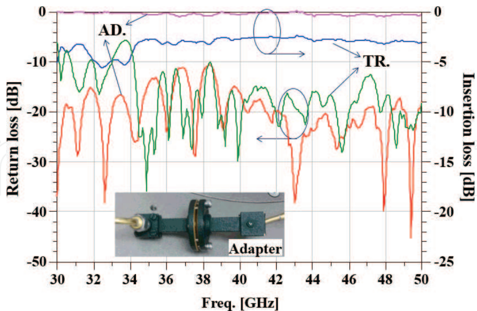
Figure 5. Measured results of the fabricated two-set transition (TR) in the back-to-back structure [an inset: an adapter connection, AD: adapters].
