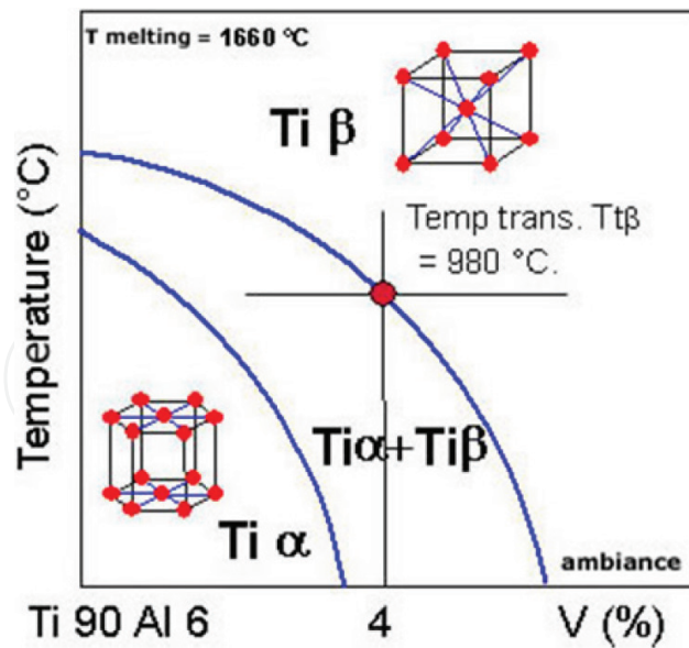
Figure 9. Schematic pseudo-binary phase diagram of TA6V4 alloy.
