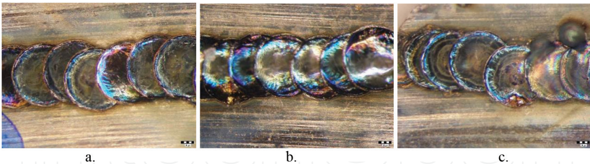
Figure 34. Macroscopic aspect of the welded CoCrMoTi5.5 alloy using different parameter values: (a) first set, (b) second set, (c) third set.
