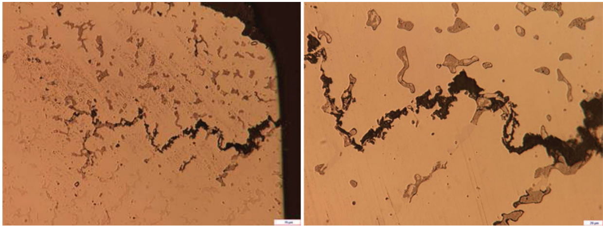
Figure 23. Microcracks in the BAA dendritic structure spread along the fragile compound precipitations, in case of fast cooling of the welded alloy.
