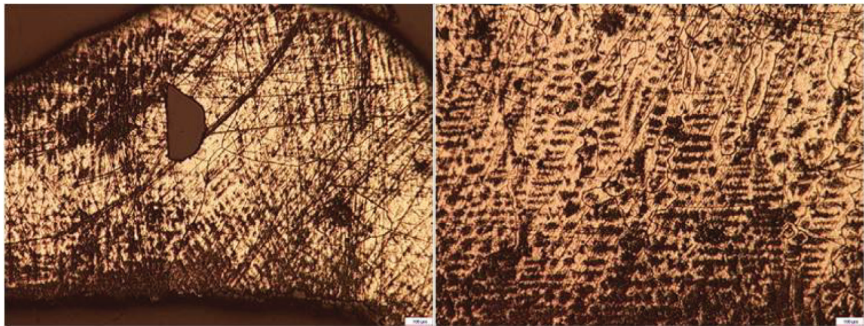
Figure 29. Metallographic aspects of pellicular intergranular precipitations, spherical shape compounds.
