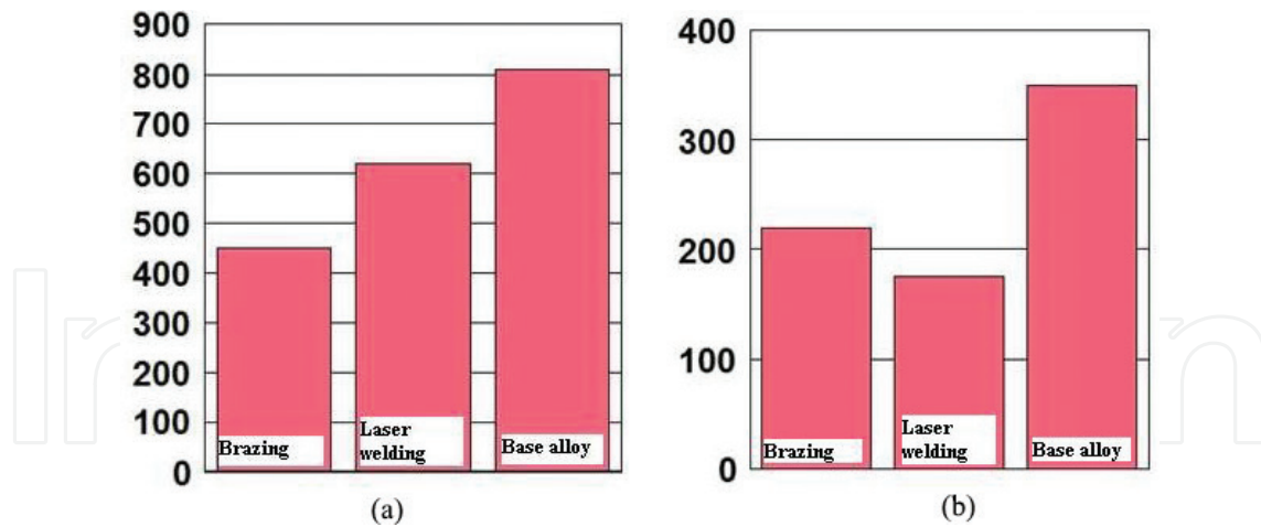
Figure 15. (a) Fracture toughness (MPa). (b) Resistance to wear (MPa).
