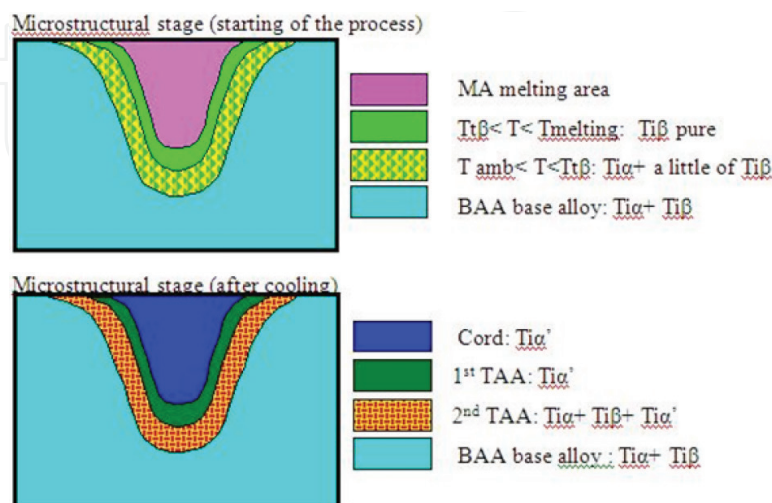
Figure 10. Schematic description of the cord during welding.
