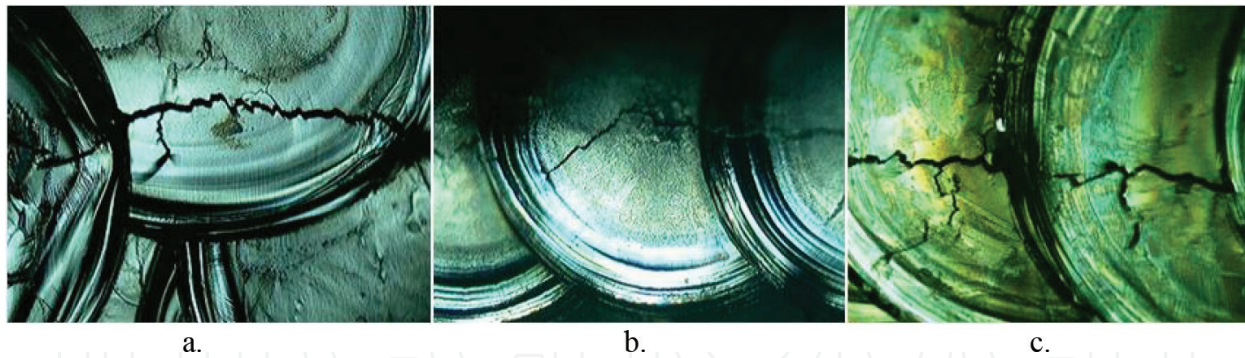
Figure 31. Microscopic aspects of “C” alloy (Vaskut Kohászati Kft) for different laser beam sizes: (a) small, (b) medium, (c) large.
