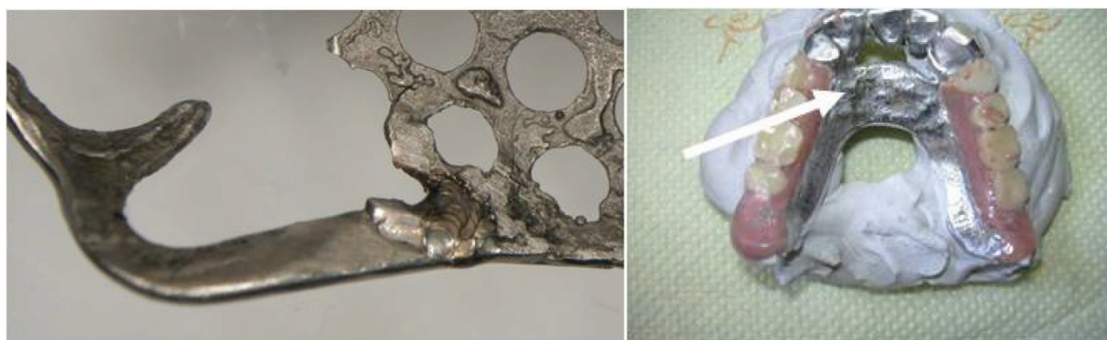
Figure 1. Laser welding of a fractured clasp and frame.
