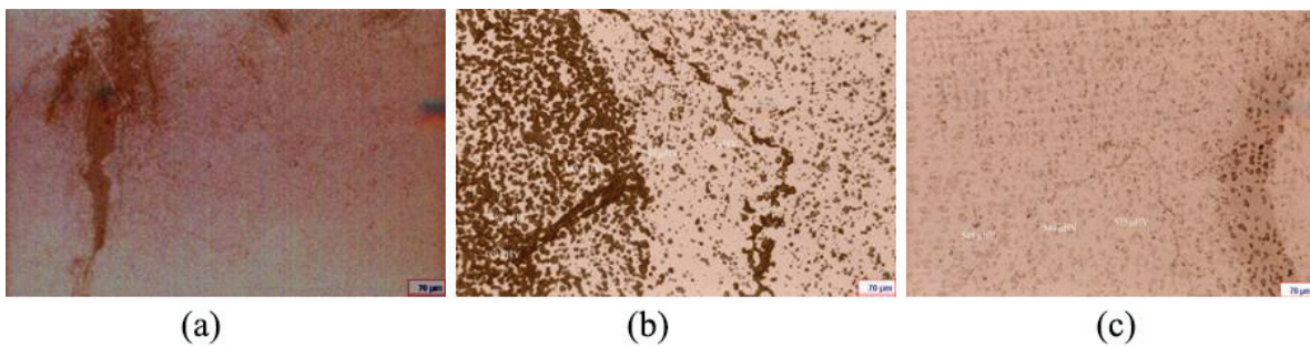
Figure 26. Microstructural aspect of Heraenium CE (Heraeus Kulzer). (a) Laser welded samples MA and TAA, microhardness values unchanged. (b) Laser welded samples without thermic treatment, MA microhardness values decreased up to 25%. (c) Micro pulse welded samples, heat treated, no microhardness changes in the TAA.
