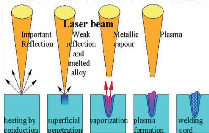
Figure 5. Stages of the welding cord formation.
