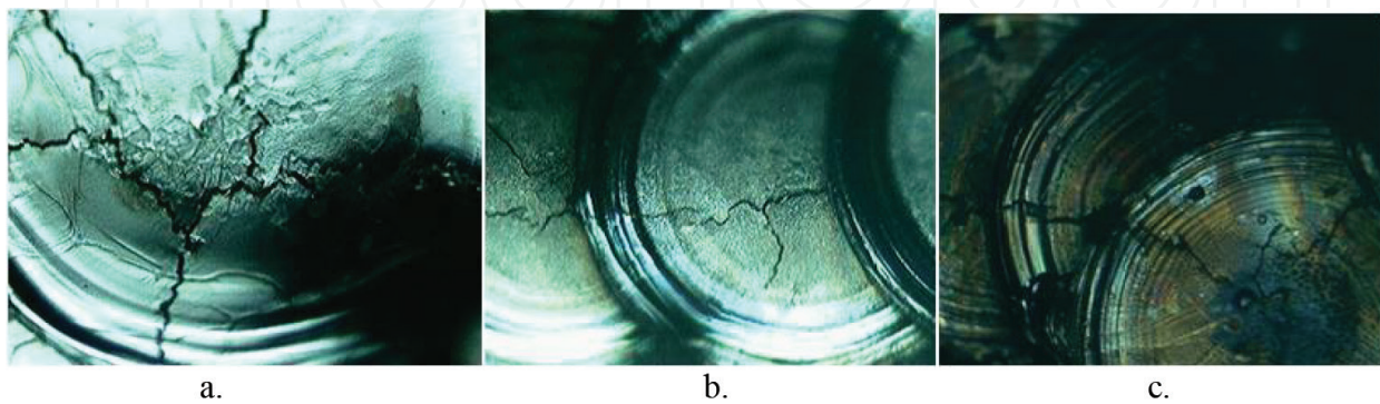
Figure 30. Microscopic aspects of Wironit extra-hard (Bego) alloy for different laser beam sizes: (a) small, (b) medium, (c) large.
