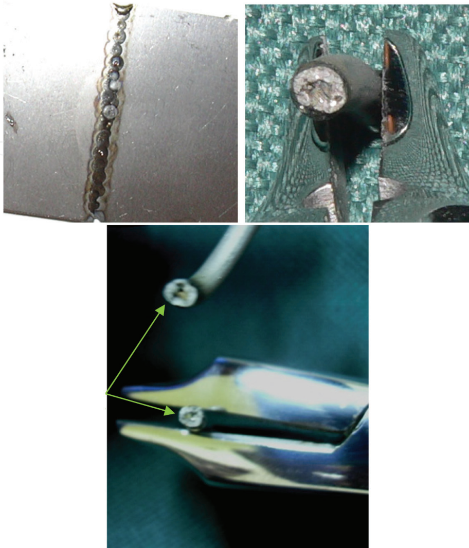
Figure 18. Laser welding without filler metal.
