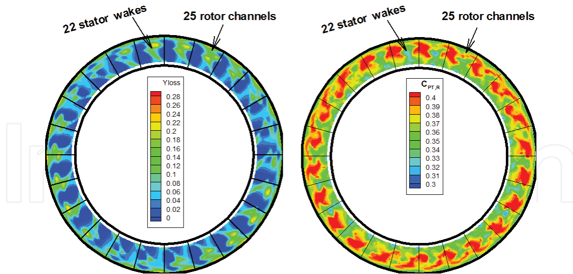
Figure 5. Rotor inlet flow field in the rotating frame of reference. Frame (a) Y_{loss} = total pressure loss. Frame (b) C_{PT,R} relative total pressure coefficient. Experiments at the Fluidmachinery Lab. at Politecnico di Milano (Italy).
