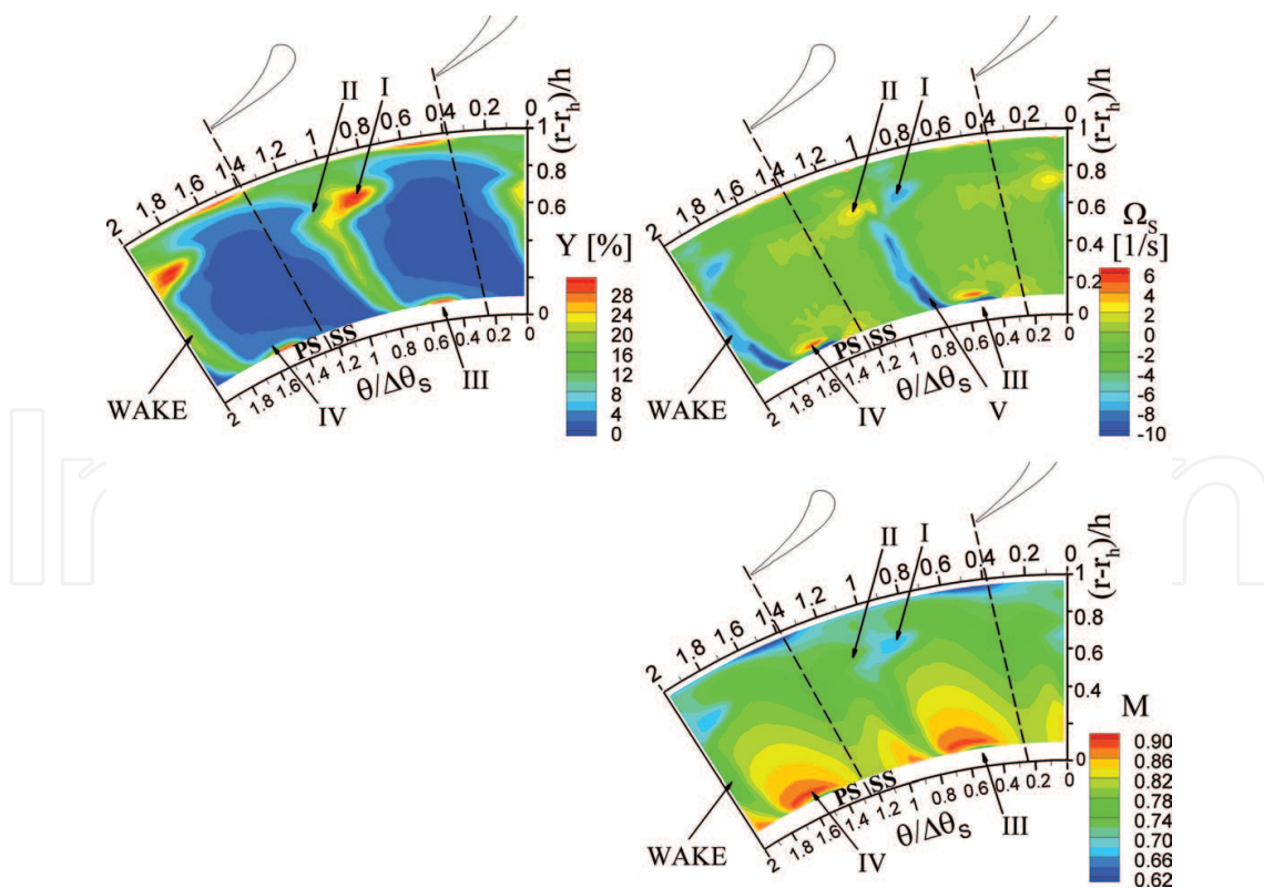
Figure 4. Total pressure loss ( Y\% ), streamwise vorticity ( \Omega_s ) and absolute Mach number ( M ) downstream of the stator. Experiments at the Fluidmachinery Lab. at Politecnico di Milano (Italy).
