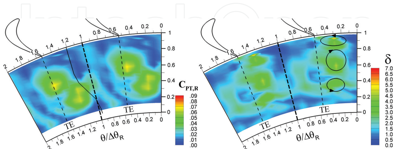
Figure 10. Standard deviation of the C_{PT,R} and \delta for the different time frames. Experiments at the Fluidmachinery Lab. at Politecnico di Milano (Italy).
