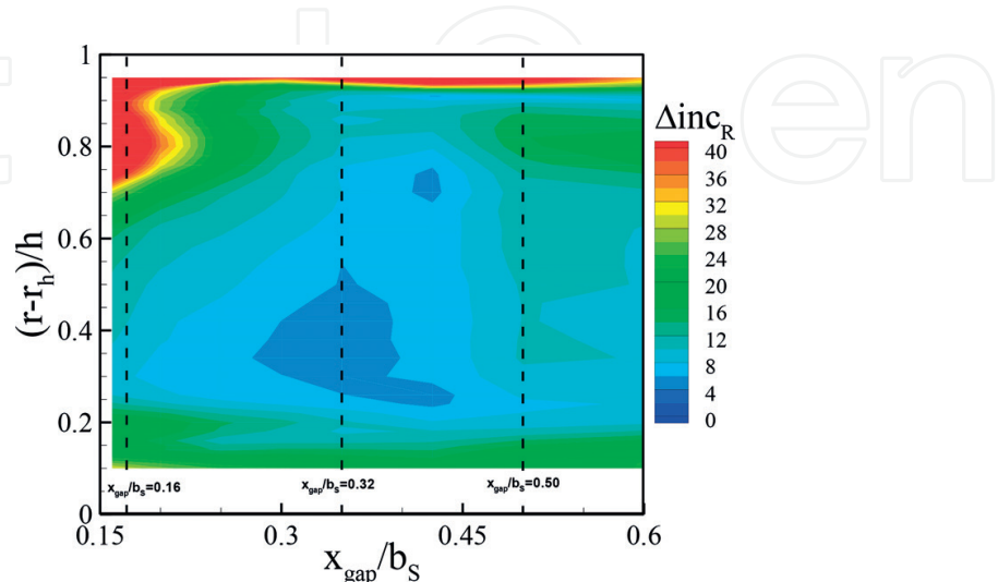
Figure 14. Rotor incidence fluctuations in circumferential direction for the different axial gaps along the blade span.
