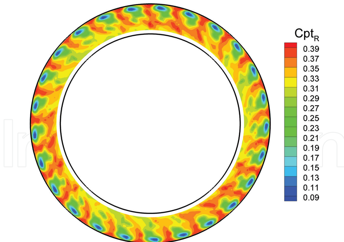
Figure 8. Relative total pressure coefficient on the whole rotor crown. Experiments at the Fluidmachinery Lab. at Politecnico di Milano (Italy).
