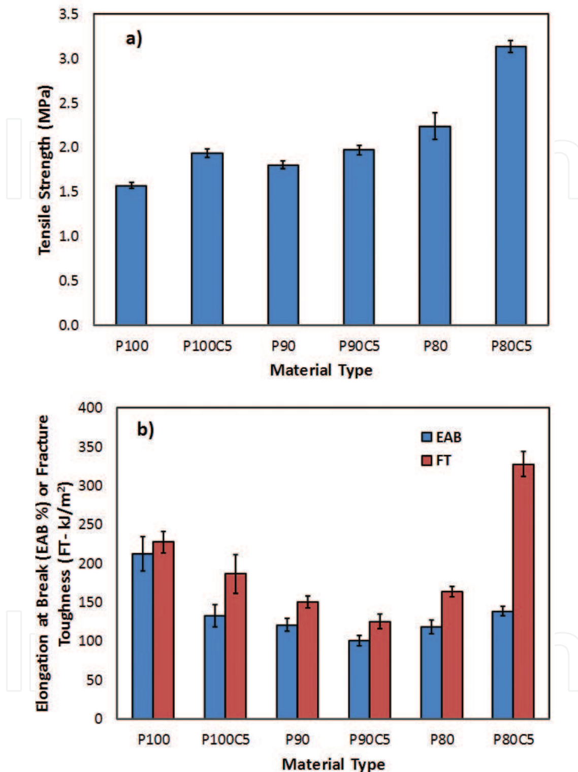
Figure 5. Mechanical properties of different electrospun fiber mats: (a) tensile strength and (b) elongation at break and fracture toughness.
