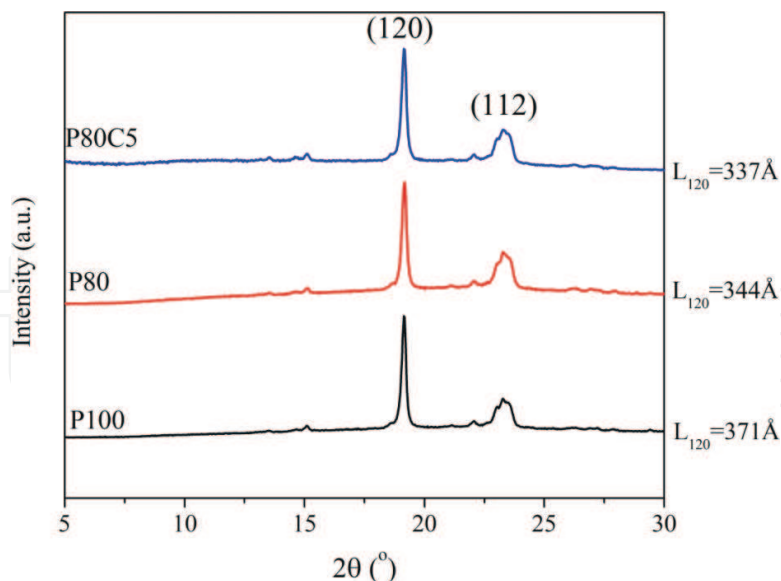
Figure 4. XRD results of different electrospun fiber mats.
