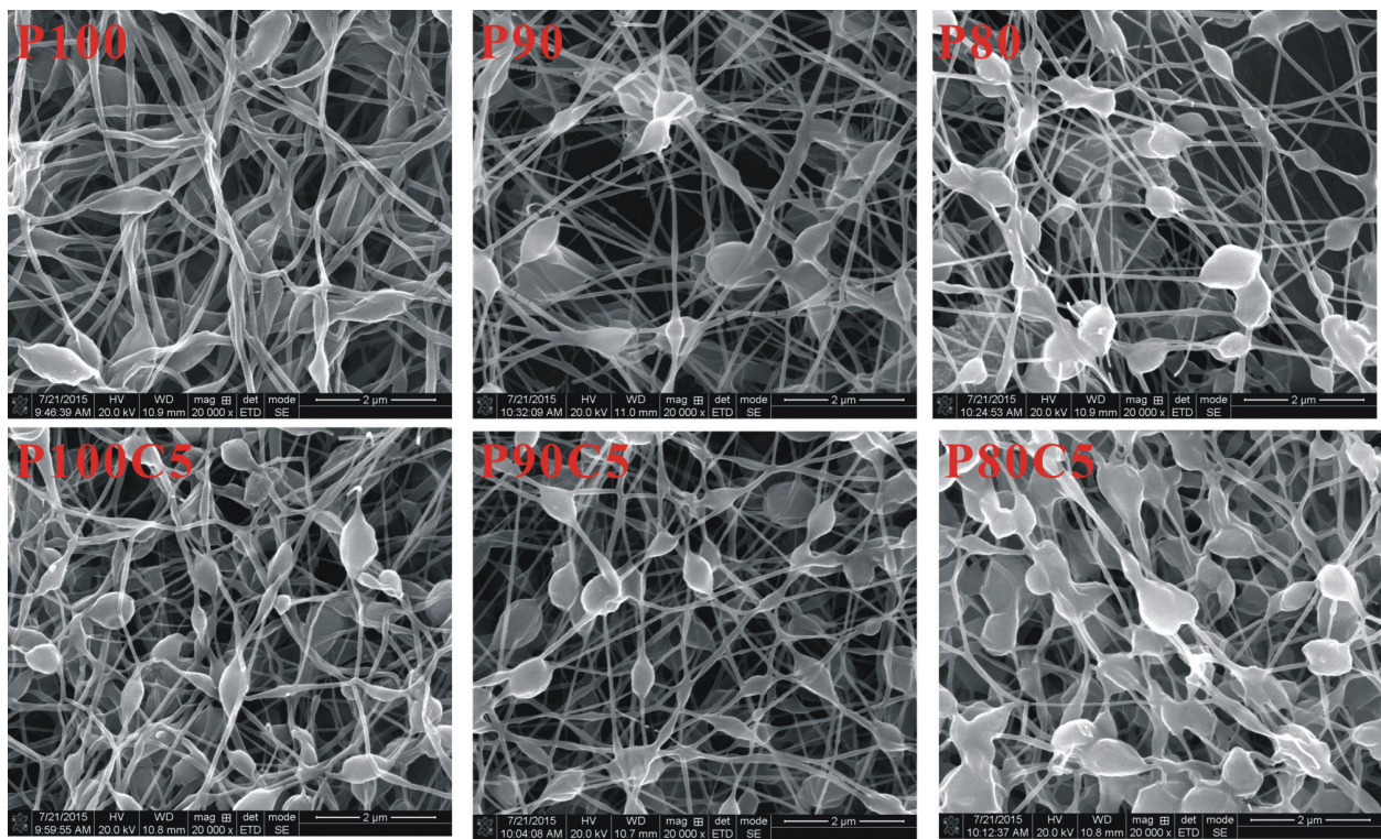
Figure 6. SEM images of different electro-spun fiber mats.
