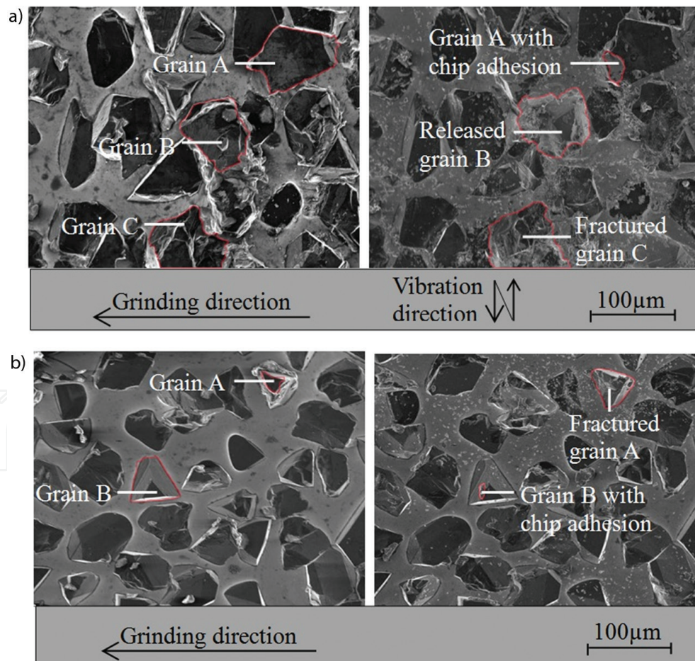
Figure 20. SEM images of the grinding wheel working surfaces before (left sides) /after (right sides) grinding of Inconel 718 (a) without and (b) with ultrasonic vibration: (a) in CG at A_{p-p} = 0 \mu\text{m} and V_c = 138.2 \text{ m/min} and (b) in UAG at A_{p-p} = 9.4 \mu\text{m} and V_c = 138.2 \text{ m/min} .
