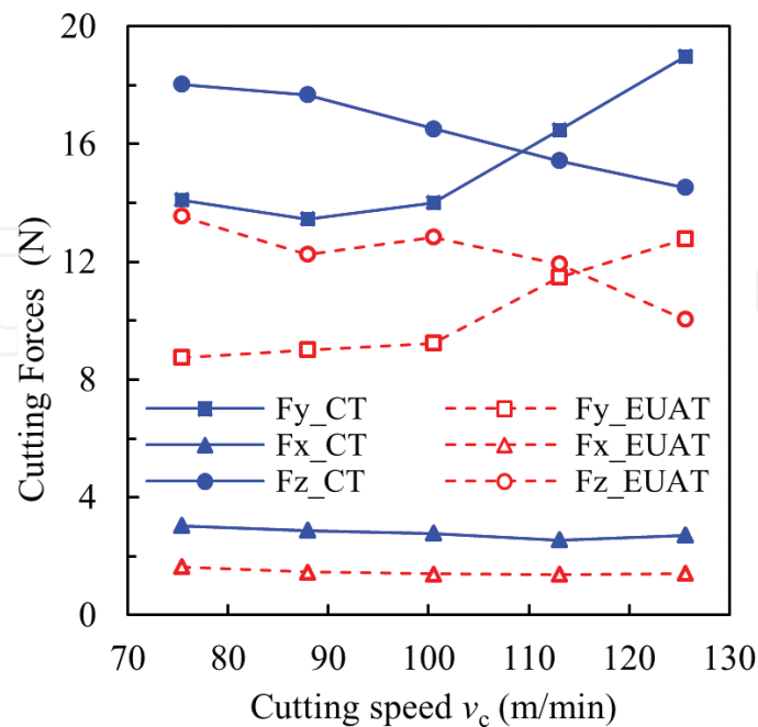
Figure 4. Effect of cutting speed on cutting forces.
