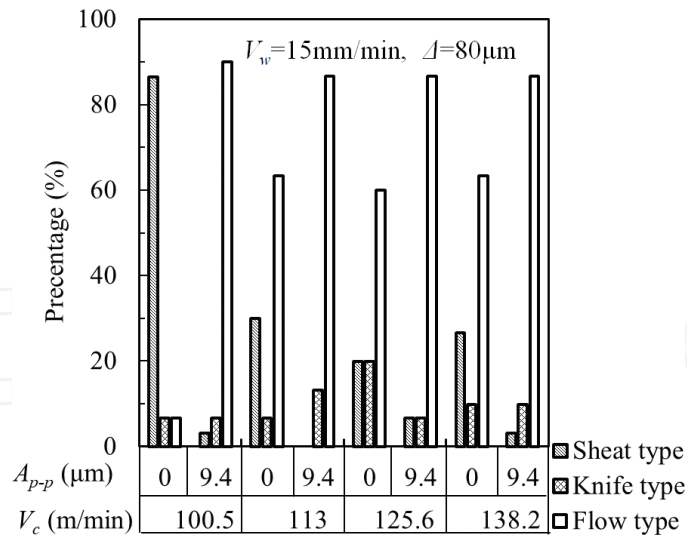
Figure 19. Effect of wheel peripheral speed on chip type.
