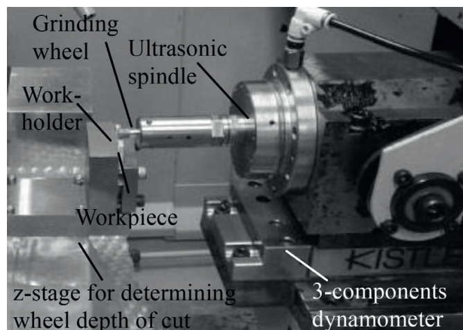
Figure 11. Photo of equipment for ultrasonic-assisted grinding.
