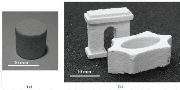
Figure 21. Manufactured ceramic objects: (a) porous filter element from corundum–zirconium ceramics produced by SLS process; (b) samples produced by SLM process from ZrO_2 powder. Reprinted from [13], with permission of Elsevier.
