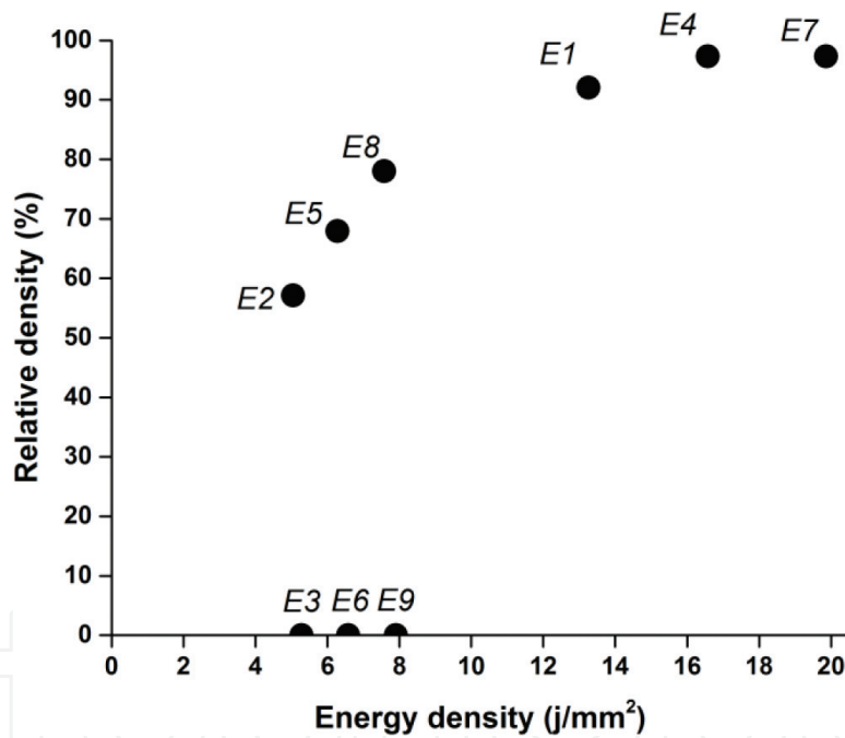
Figure 8. Relative density of laser produced part vs. laser energy density. The data presented here are extracted from those presented in the original source [28].
