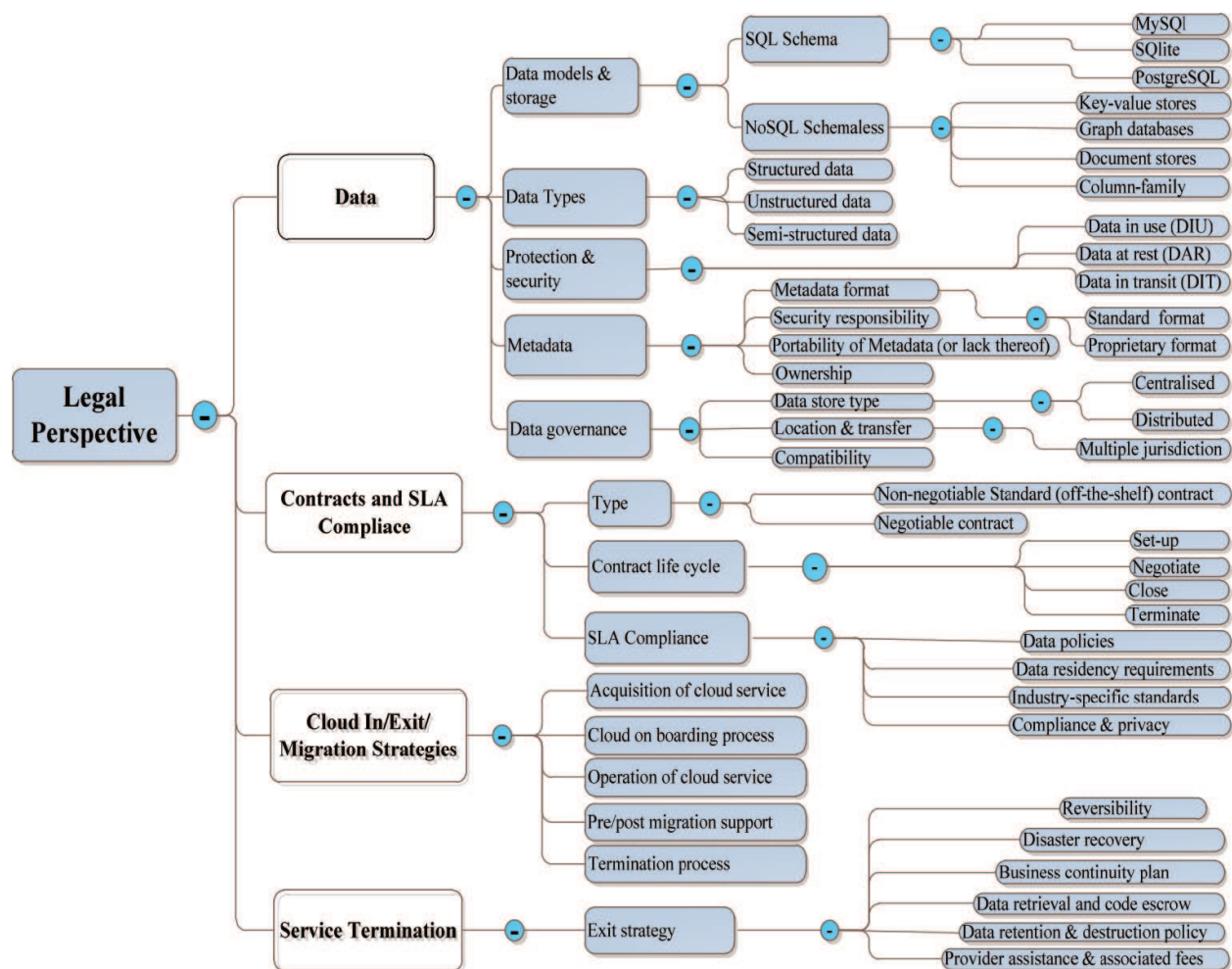
Figure 4. Vendor lock-in taxonomy – legal perspective.
