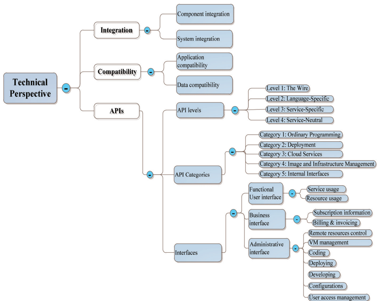
Figure 3. Vendor lock-in taxonomy – technical perspective.
