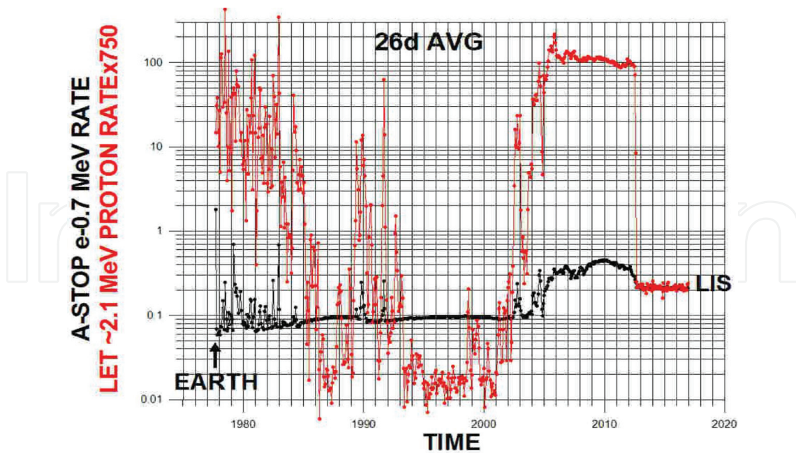
Figure 2. Same as Figure 1 . The L1-L2 stop 1.8–2.6 MeV proton rate (in red) is normalized to the A-stop 0.7 MeV LIS electron rate using the factor \times 750 .
