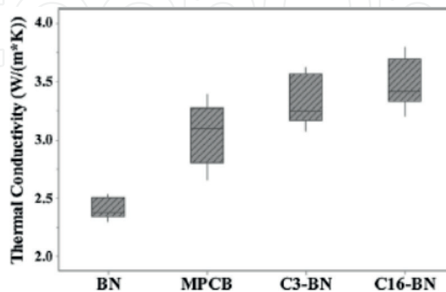
Figure 9. Thermal conductivities of h-BN/epoxy composites with untreated BN, MPCB ( \text{Al}_2\text{O}_3 /epoxy), silane (C3)/BN, and silane (C16)/BN [23].
