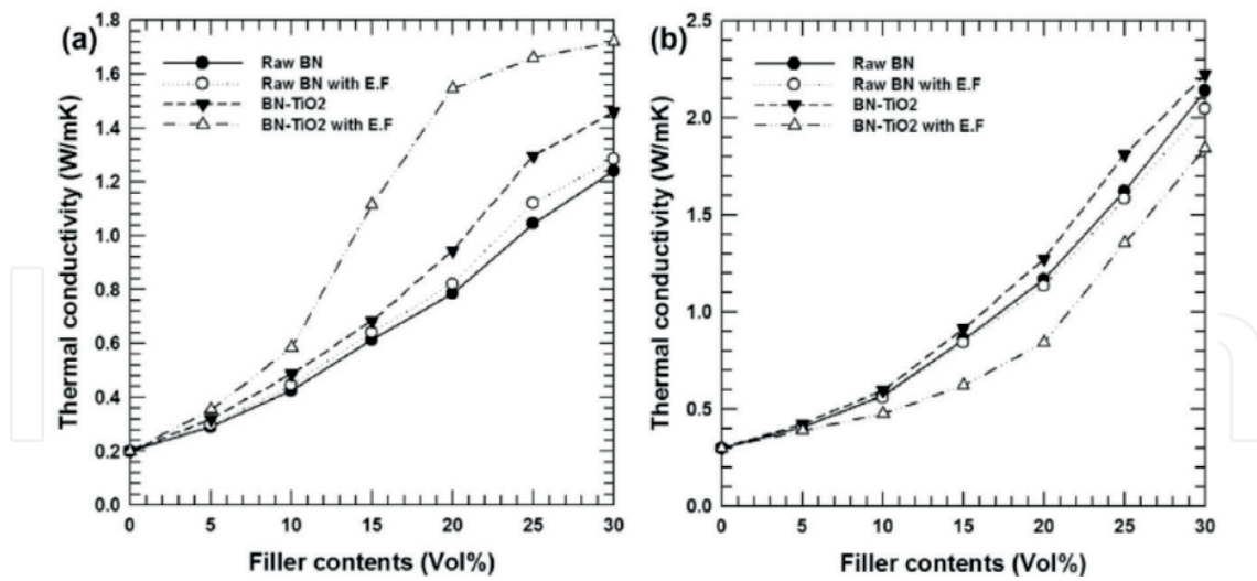
Figure 7. Thermal conductivity of h-BN/PUA composite and \text{TiO}_2 coated h-BN/PUA composite before and after electric field alignment: (a) through-plane and (b) in-plane thermal conductivity [21].
