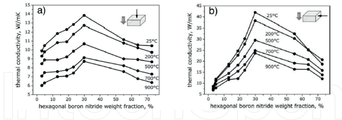
Figure 4. Compositional dependence of thermal conductivity of the composites in the ( \gamma -AlON)-BN system determined in (a) perpendicular and (b) parallel to the pressing force [20].
