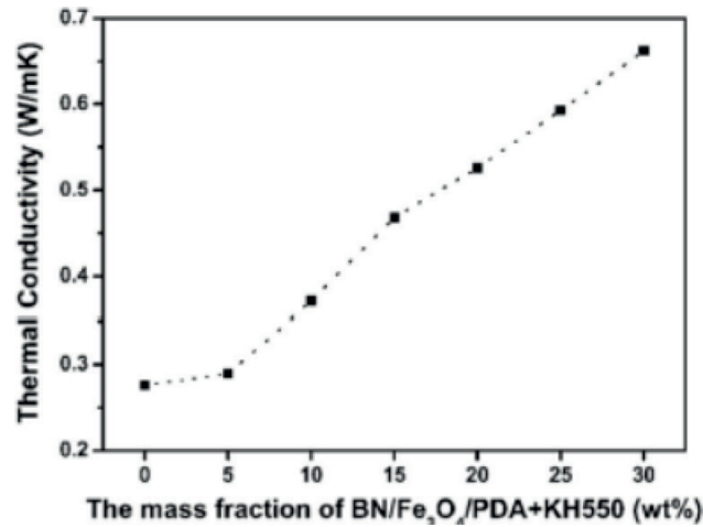
Figure 8. Thermal conductivities of neat PEN and BN/ \text{Fe}_3\text{O}_4 /PDA + KH550/PEN composite films with various amounts of filler loading content [22].
