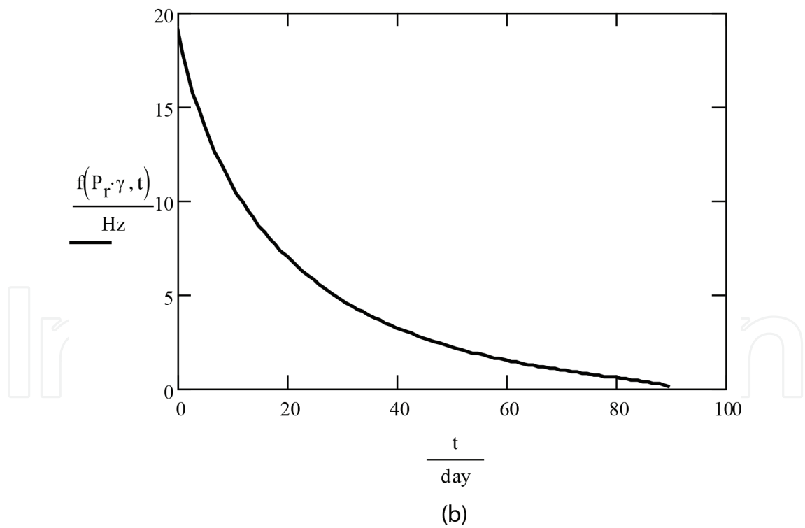
Figure 6. Frequency of the beam with time with viscoelasticity. (a) Frequency with time for capacity of the section, (b) Safety factor \gamma —Collapse at 90th day.
