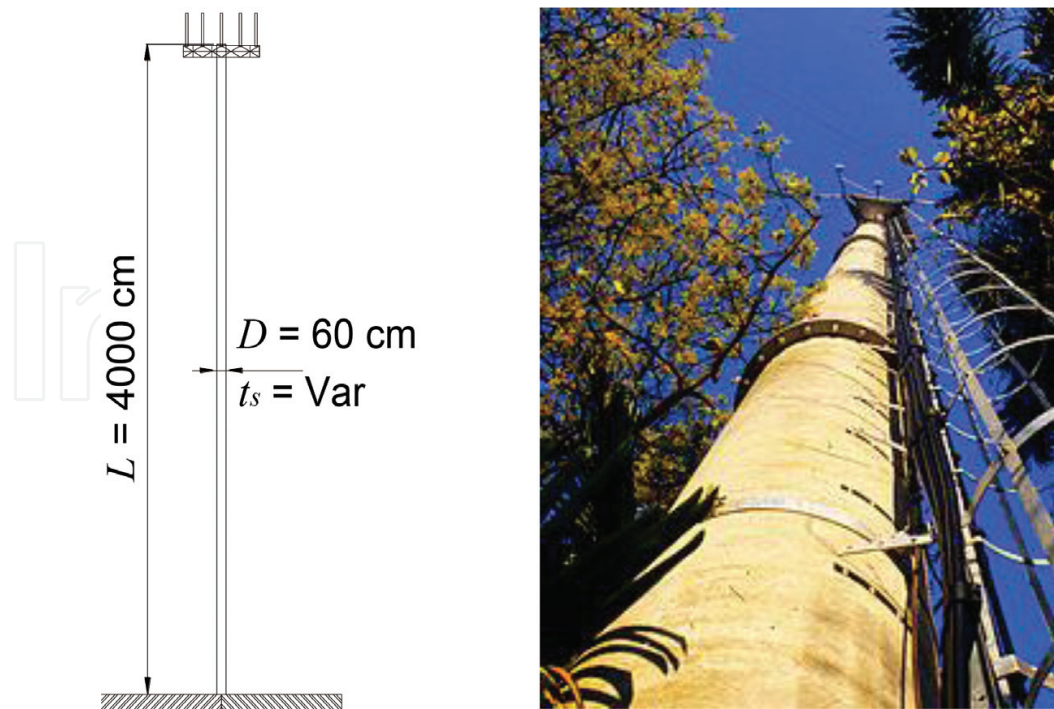
Figure 9. A column as a mast transition system.
