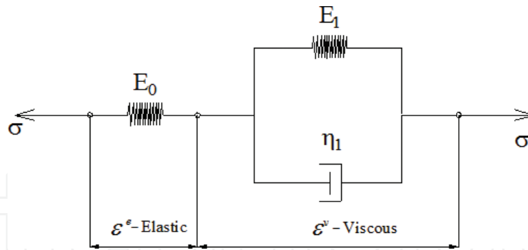
Figure 1. Viscoelastic model of three parameters.
