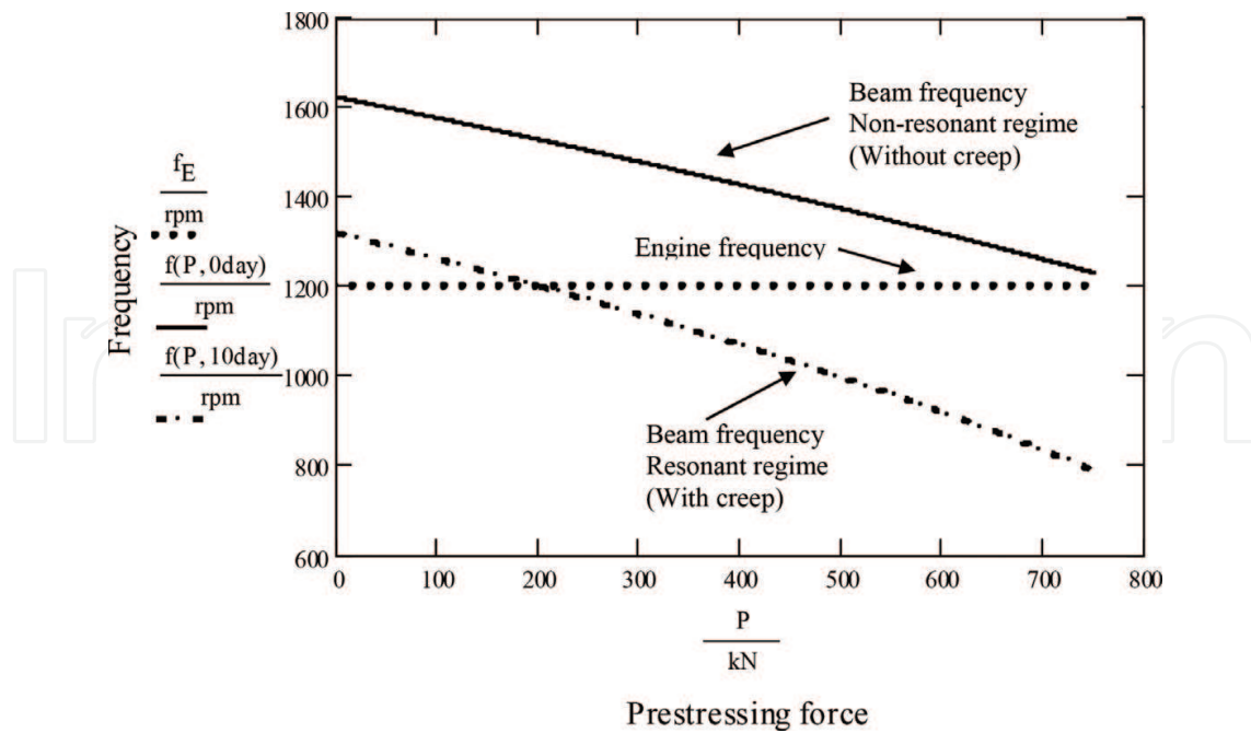
Figure 7. Resonant and non-resonant frequencies as a function of axial compression force P .
