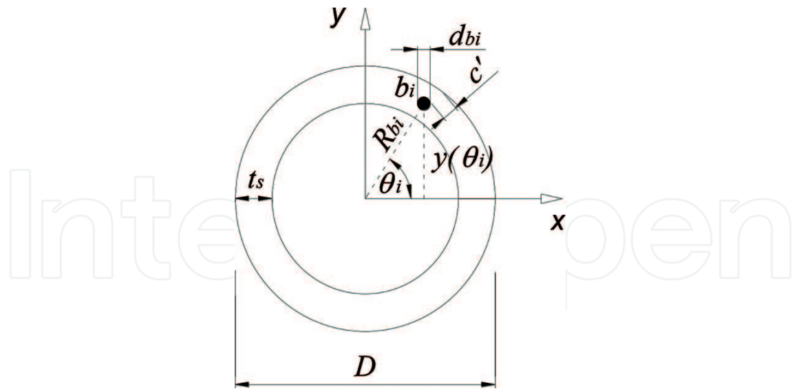
Figure 11. Parameters for homogenizing concrete section.
