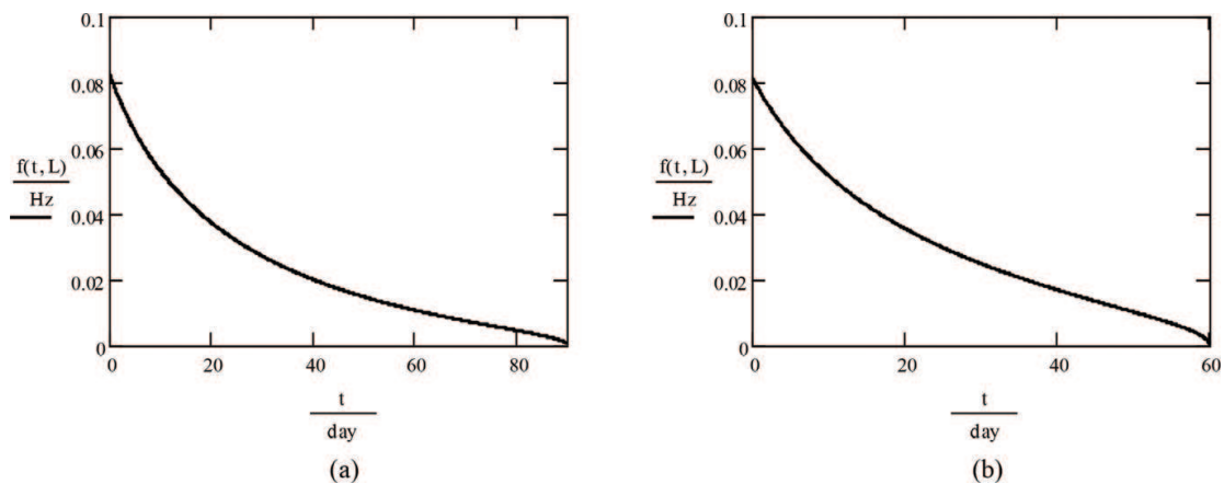
Figure 13. Structural frequency on height of losing stability. (a) L = 50.6975 m—Collapse on the 90th day, (b) L = 57.0000 m—Collapse on the 60th day.
