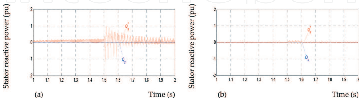
Figure 10. Stator reactive power (pu): (a) conventional single RCS, (b) proposed dual RCS.
