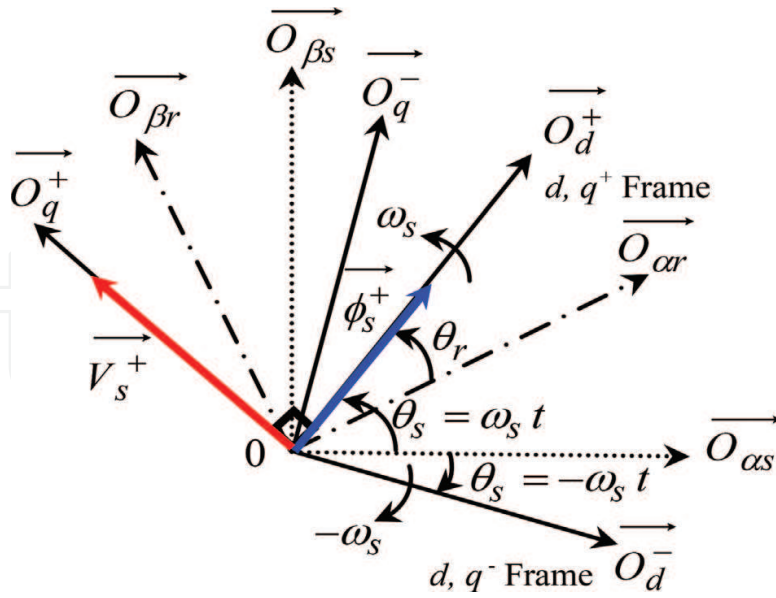
Figure 5. Stator flux orientation under unbalanced grid.
