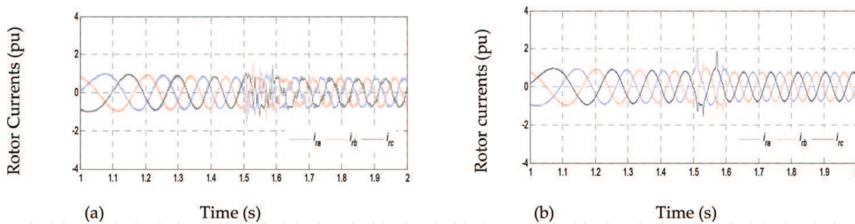
Figure 16. Rotor currents (pu): (a) conventional single RCS, (b) proposed RCS.
