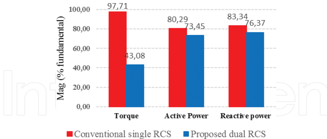
Figure 19. Comparison of ripples in electromagnetic torque, stator active and reactive power between the two control strategies.
