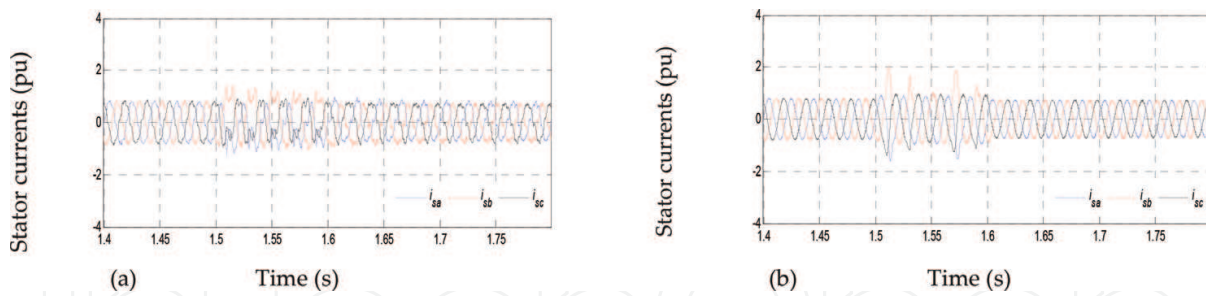
Figure 14. Stator currents (pu): (a) conventional single RCS, (b) proposed dual RCS.
