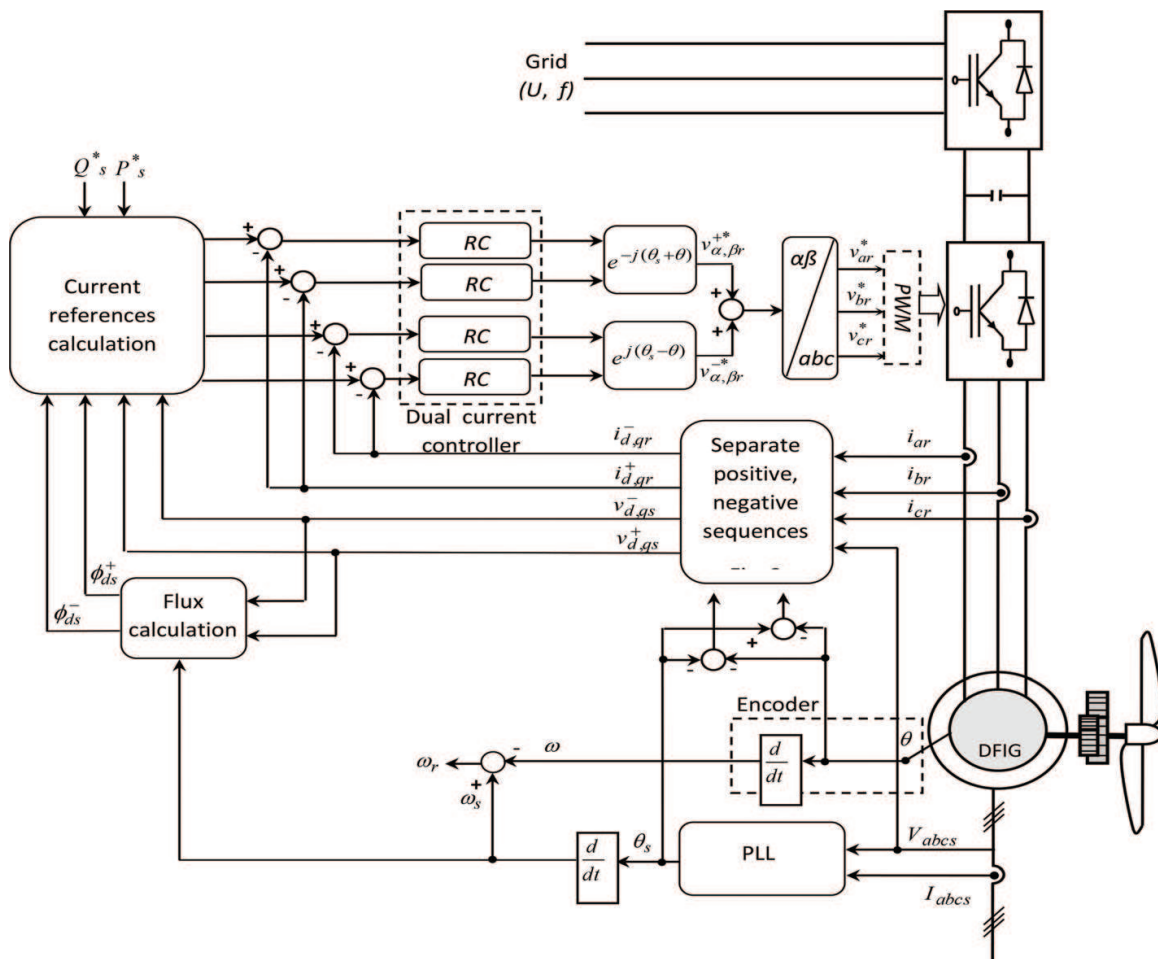
Figure 6. Block diagram of the proposed Lyapunov-based robust control scheme.
