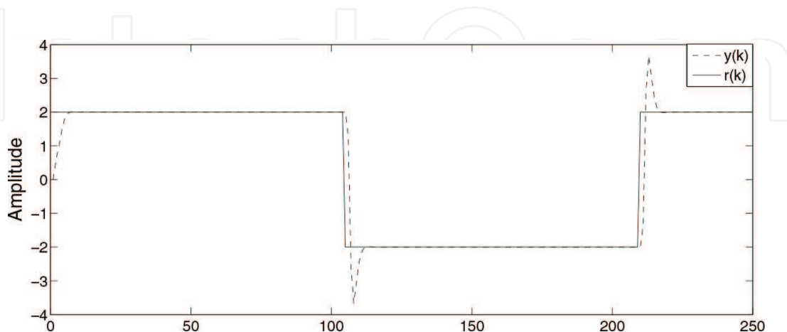
Figure 4. Output signal: PID-pole placement method.
