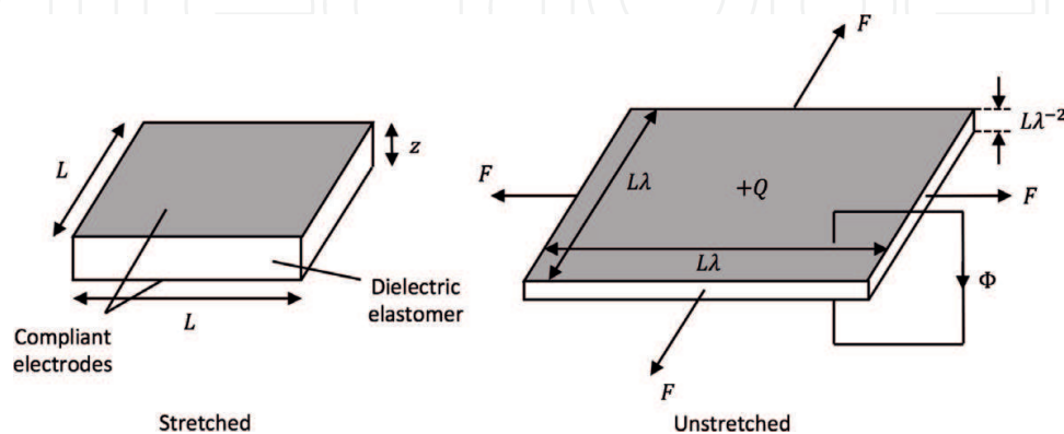
Figure 5. Loading of a dielectric elastomer.
