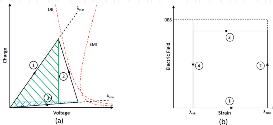
Figure 4. More recent energy harvesting schemes. (a) The optimised scheme. (b) Constant field scheme.
