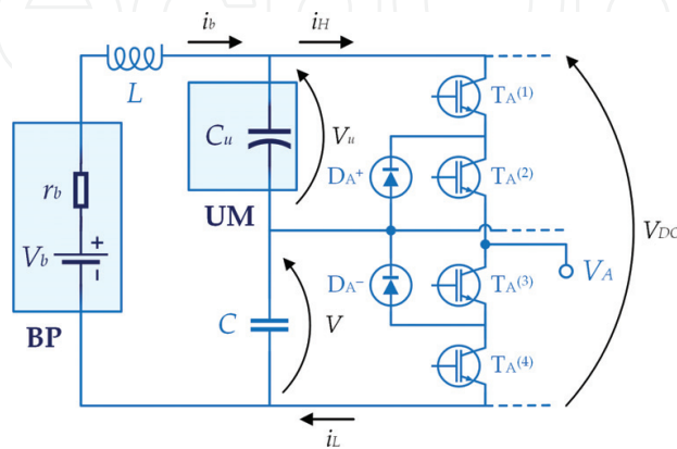
Figure 6. The highly integrated HESS configuration proposed in [31–33].
