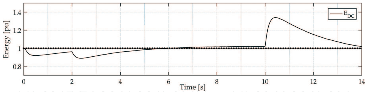
Figure 20. DC-link energy variations.
