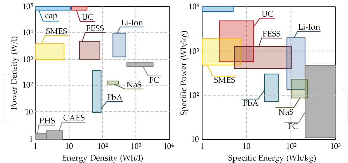
Figure 2. Energy/power density (left) and specific energy/power (right) of ESSs on Ragone plots: pumped hydroelectric storage system (PHS), compressed air energy storage system (CAES), and fuel cell (FC).
