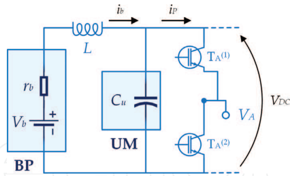
Figure 3. Schematic representation of passive HESS configuration.
