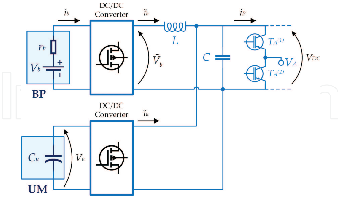
Figure 4. Schematic representation of active parallel HESS configuration.
