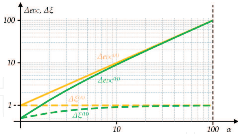
Figure 8. The evolutions of both \Delta \xi (dashed lines) and \Delta e_{DC} (solid lines) with \alpha : active and HIBUC configurations.
