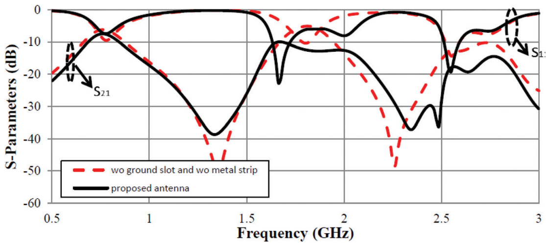
Figure 5. S-parameters of the proposed antenna without any isolation techniques and with both the techniques.
