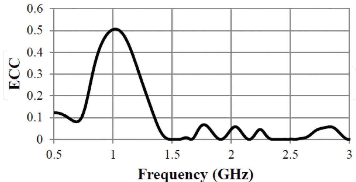
Figure 11. Variation of ECC with frequency.
